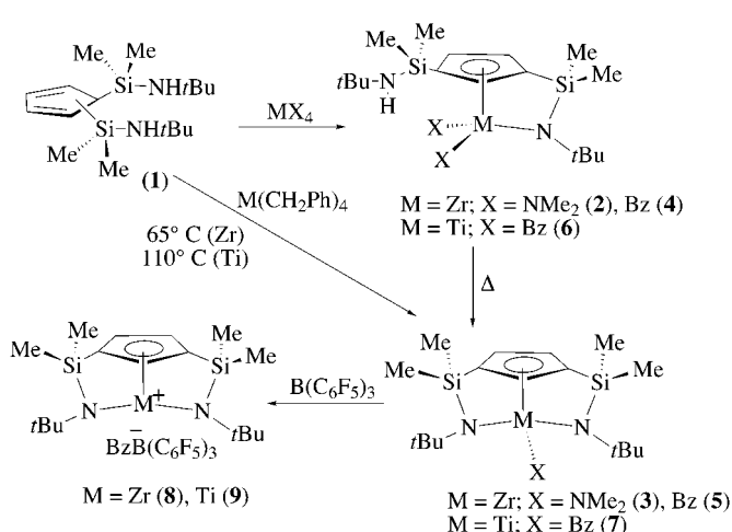
Scheme 1. Synthesis of neutral bridged \eta^5 -cyclopentadienyl mono- and di( \eta -amidodisilyl)titanium and -zirconium complexes and their cationic species.
