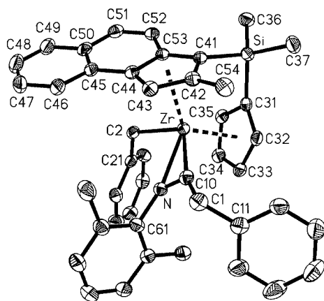
Figure 3. Ellipsoid plot of compound 6 (50% probability level); hydrogen atoms have been omitted for clarity
