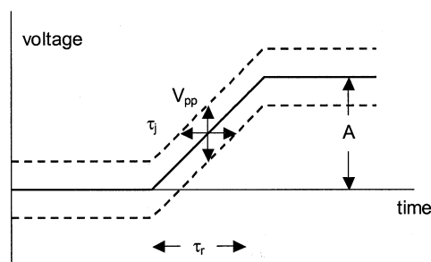
Fig. 1. Simple theory of RFI-induced jitter.
