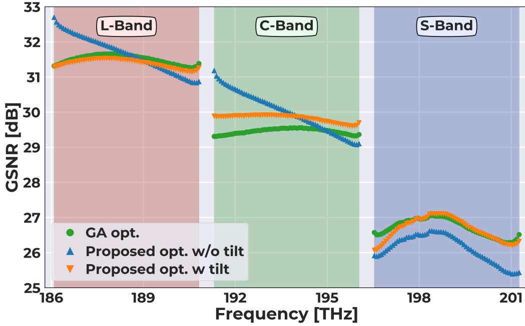
Fig. 4.19 GSNR profile for C+L+S scenario using 64 GBaud and 75 THz of symbol rate and WDM grid, respectively, comparing the power optimization using the GA and the proposed method without and with applied tilt.
