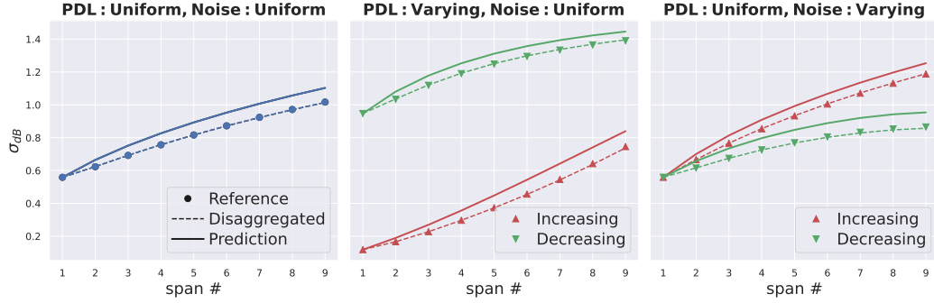
Fig. 3.20 OSNR PDL-induced \sigma simulated and evaluated with the proposed methodology for all the investigated transmission scenarios.
