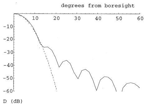
— theoretical pattern for corrugated horn of aperture diameter 4\lambda (after [15]) --- (\cos \theta)^n curve fit (where n = 208 )
