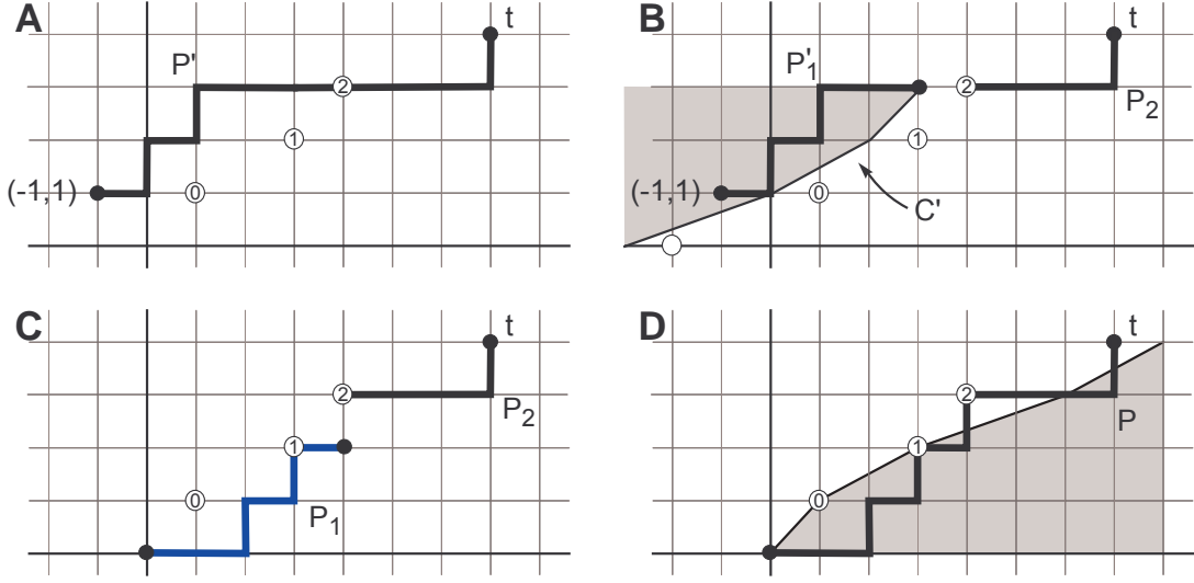
FIGURE 8. Construction of \phi_j : \mathcal{W}^j \longrightarrow \mathcal{B}_i^j , with \mathbf{a} = (1, 2, 3, 2) , i = 4 , j = 2 , and s_i = 2 . The point b_i^j is indicated with a circled j , and b_i^{-1} with an open circle. The boundary curve in panel D is \partial \mathbf{a}^{(s_i+j)} = \partial \mathbf{a}^{(4)} .
