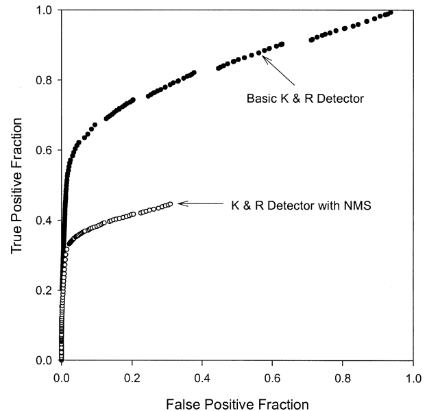
Fig. 3. ROC plots for the basic and nonmaximally suppressed KR detector.
