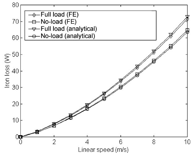
Fig. 15. Variation of iron loss with speed (1.5-kW machine).
