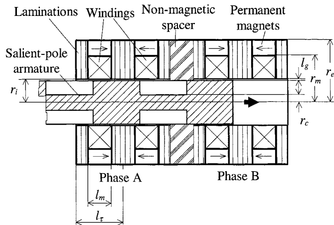
Fig. 1. Schematic of two-phase tubular permanent-magnet generator.
