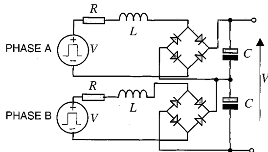
Fig. 2. Rectification and energy storage circuit.
