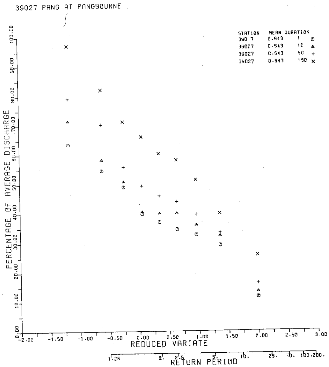
FIGURE 1.3 AUTOMATED FLOW FREQUENCY PLOT FOR RIVER PANG
