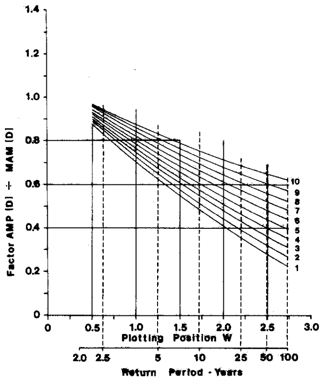
FIGURE 3.3 FLOW FREQUENCY TYPE CURVES
