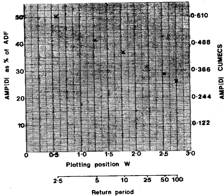
FIGURE 3.4a FLOW FREQUENCY CURVE FOR PANG FOR D = 60 DAYS FROM CATCHMENT CHARACTERISTICS
