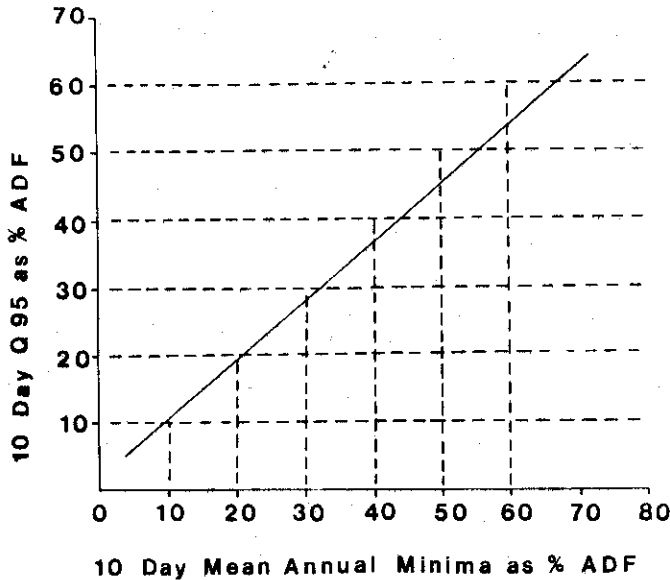
FIGURE 4.1 APPROXIMATE FLOW DURATION : FLOW FREQUENCY RELATION
