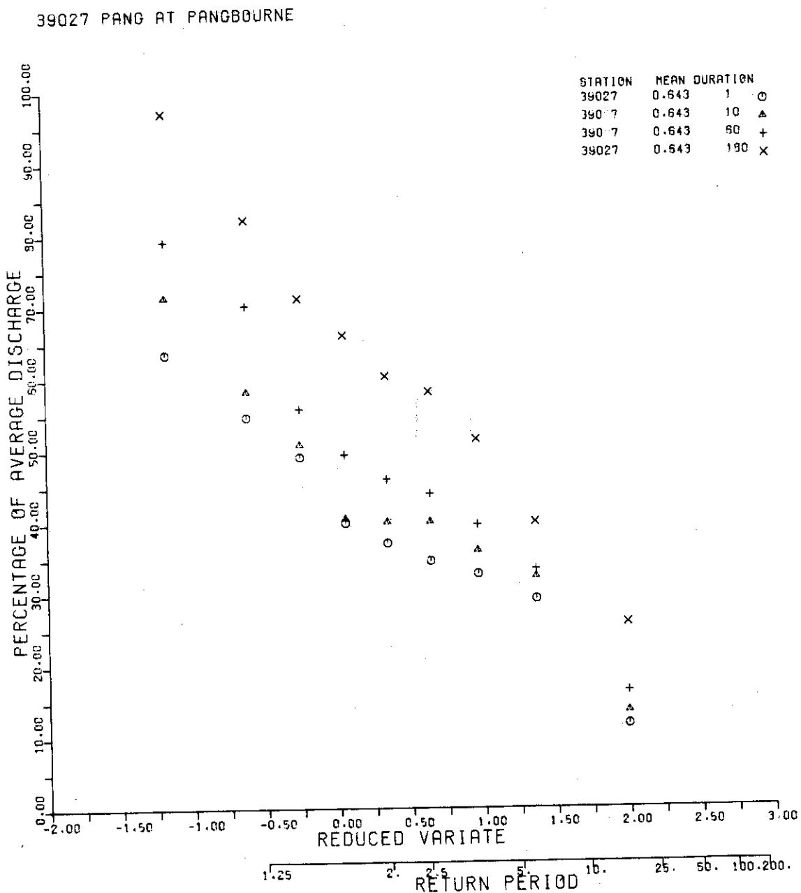
FIGURE 2.2a FLOW FREQUENCY CURVE FOR PANG
