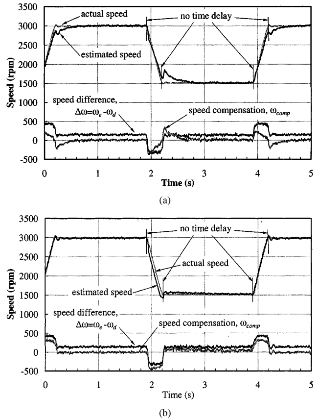
Fig. 9. Performance of improved speed estimation method. (a) Time constant T = 10 s. (b) Time constant T = 100 s.
