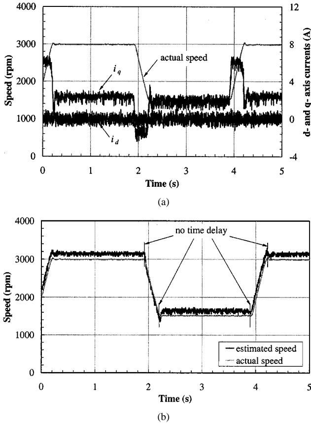
Fig. 8. Estimation of speed from EMF and excitation flux. (a) d -axis and q -axis currents, rich of noise. (b) Comparison of estimated and actual speed.
