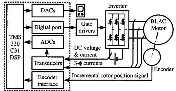
Fig. 1. Block diagram of DSP-controlled BLAC drive system.
