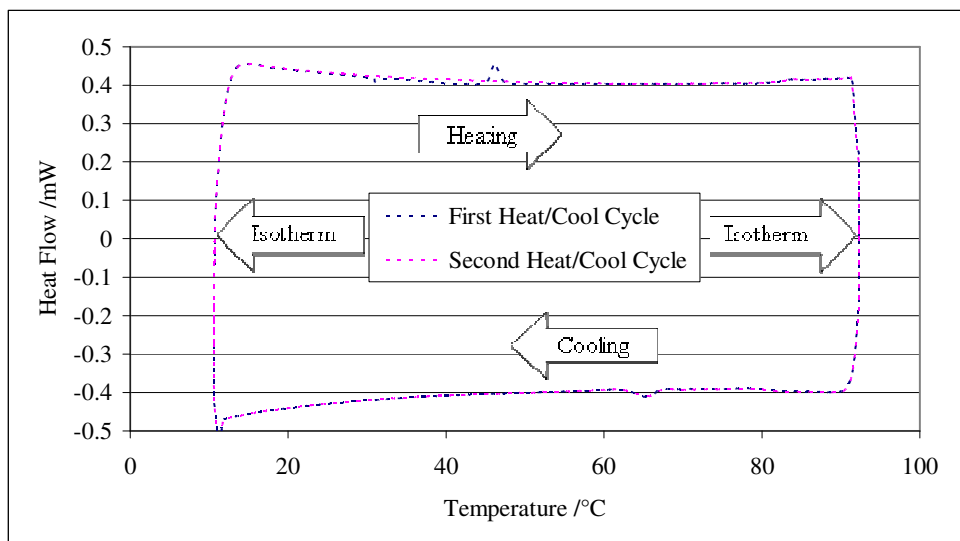
Figure 5 DSC trace of 1.9 g l -1 PA sample being heated and cooled at 0.5 °C min -1
