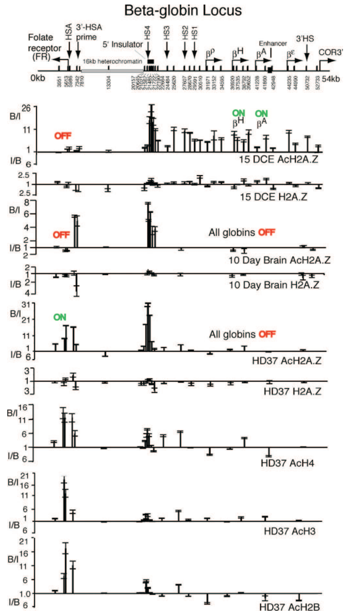
Figure 4. Distributions of H2A.Z, Ach2A.Z, Ach4, Ach3 and Ach2B at the \beta -globin locus/folate receptor gene in 15-day chicken erythrocytes (15DCE), 10-day chicken brain tissue (10DCB) and HD37 chicken erythroblasts. Nomenclature as in Figure 3. B/I values (the ratio of the Bound to the Input signal for an amplicon) above the unity lines represent 'fold enrichment' achieved by the antibodies. I/B values are plotted below the unity lines when the Bound signal is less than that of the Input: this ratio represents 'fold depletion'.
