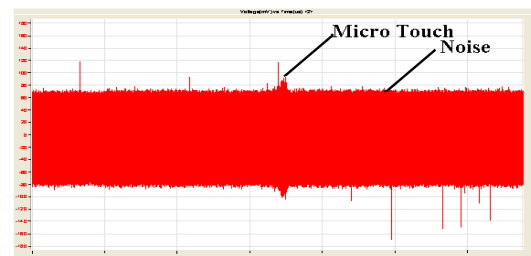
Figure 2: Raw signal showing micro-touch detected by AE sensor
