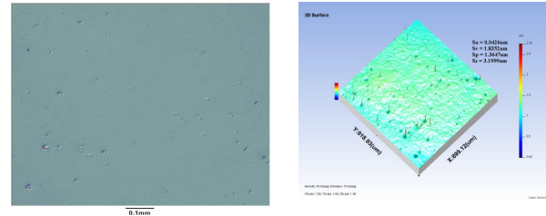
Figure 1: White light interferometer surface topography of Inconel 718 before micro-touch
