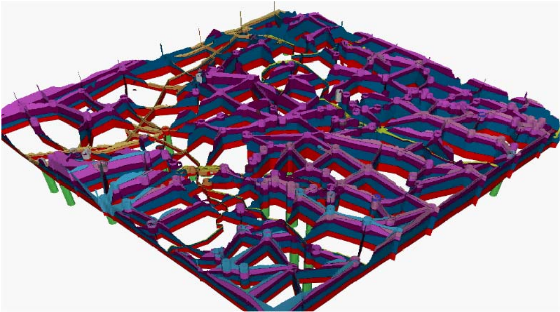
Figure 5. Fence diagram generated from the borehole database.
