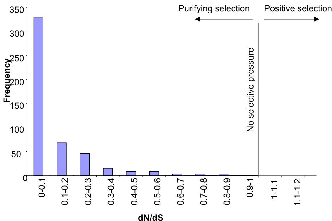
Figure 5 Distribution of dN/dS ratios among Ancylostoma ortholog pairs. dN and dS are the rates of nonsynonymous and synonymous amino acid substitutions, respectively.
