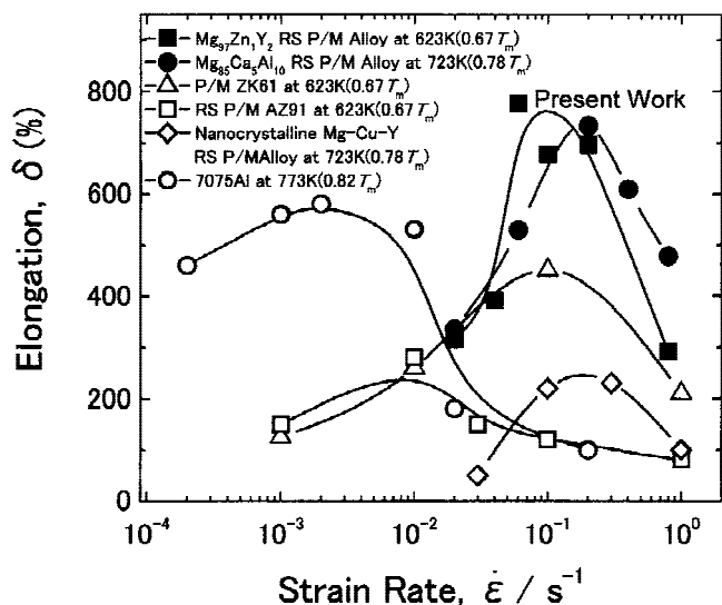
FIG. 5. Relation between \delta and strain rate for the RS/PM \text{Mg}_{97}\text{Zn}_1\text{Y}_2 alloy produced at T_e = 573 \text{ K} . The data of other conventional metallic alloys are also shown for comparison.
