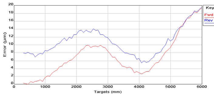
Figure 6: Effect of temperature change on linear positioning
