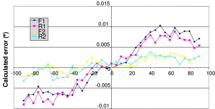
Figure 11: A-axis positioning error with W-axis retracted and fully extended
