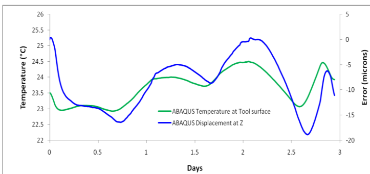
Figure 20: Simulated temperature and displacement profiles recorded over 3 days at mandrel's Z axis
