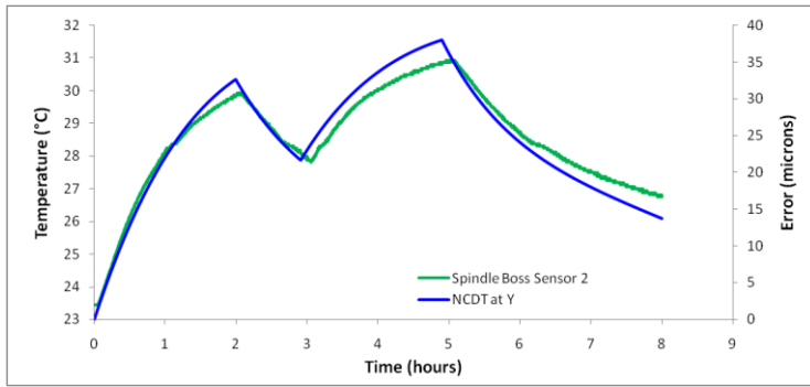
Figure 16: Experimental temperature and displacement profiles step heat and cool cycles
