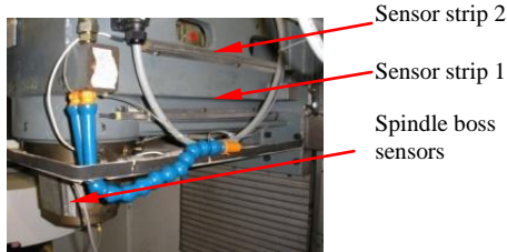
Figure 7: Thermal sensors location on the machine
