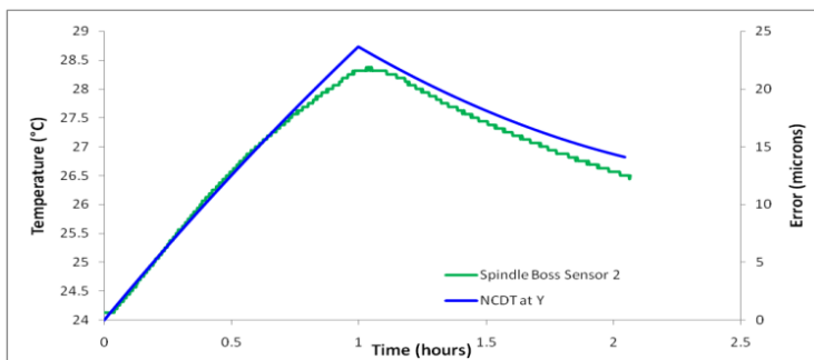
Figure 12: Experimental temperature and displacement profiles for 1 hour heat and 1 hour cooling cycle
