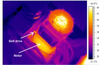
Figure 8: Thermal distribution (top) showing spindle motor and belt drive
