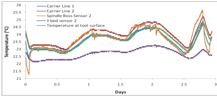
Figure 18: Environmental temperature variations recorded over 3 days
