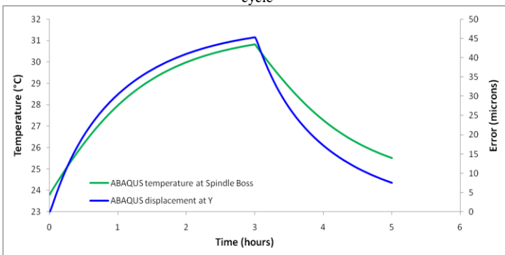
Figure 15: Simulated temperature and displacement profiles for 3 hour heat and 2 hour cooling cycle
