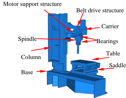
Figure 6: Halved model (Symmetry)
