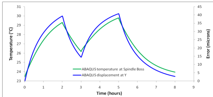
Figure 17: Simulated temperature and displacement profiles for step heat and cool cycle
