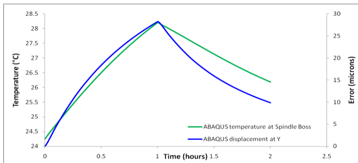
Figure 13: Simulated temperature and displacement profiles for 1 hour heat and 1 hour cooling cycle
