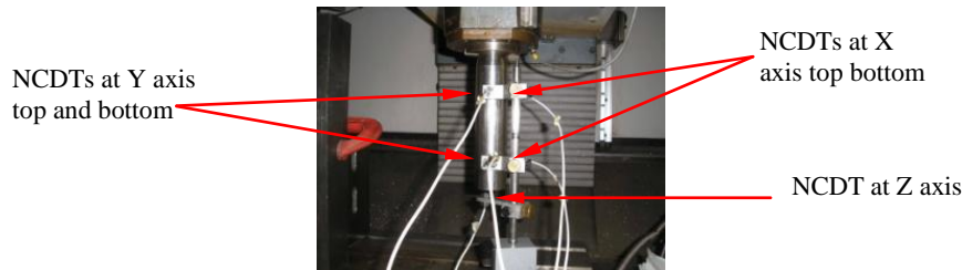
Figure 9: NCDTs located around the tool
