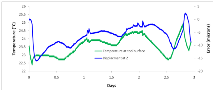
Figure 19: Experimental temperature and displacement profiles recorded over 3 days at mandrel's Z axis
