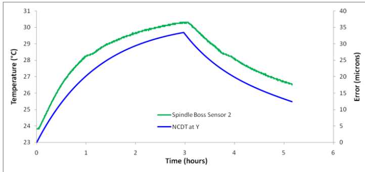
Figure 14: Experimental temperature and displacement profiles for 3 hour heat and 2 hour cooling cycle
