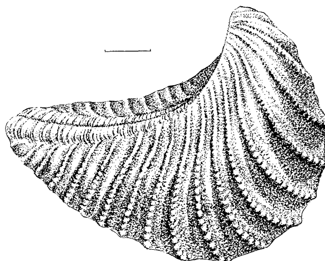
Fig. 4 Pterotrigonia bungoensis Tashiro and Tanaka (scale 10 mm)
