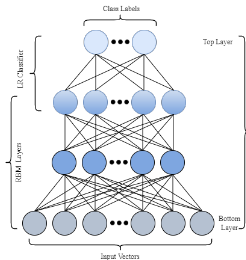
Figure 14. Architecture of a deep belief network (DBN) [101].
