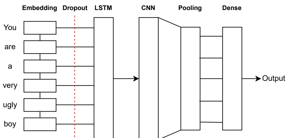
Figure 19. LSTM-CNN Model Architecture
