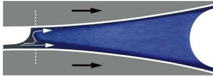
FIGURE 10. Dye trace showing the absence of a primary transfer jet and that transfer of fluid to the upper roll is entirely by means of the secondary transfer jet ( R/H_0 = 100 , S = 1.0 , \lambda_i = 0.29 , Ca_2 = 2.78 \times 10^{-2} ).
