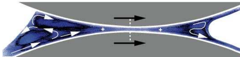
FIGURE 12. 'Fully' flooded forward roll coating with an upstream bank and two saddle points (indicated by +) marking the onset of regions of recirculating flow ( R/H_0 = 200 , S = 0.69 , \lambda_i = 1.08 , Ca_2 = 9.83 \times 10^{-2} ). Flow-back occurs at the inlet since only part of the incoming flow can pass through the nip.
