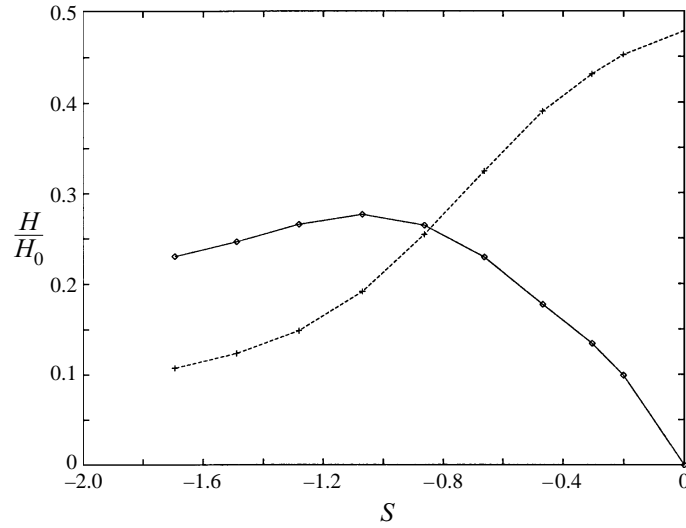
FIGURE 22. Non-dimensional film thicknesses (◇, H_1/H_0 ; +, H_2/H_0 ) as a function of S for reverse-mode coating ( R/H_0 = 100 , \lambda_i = 0.24 , Ca_2 = 2.05 \times 10^{-2} ).
