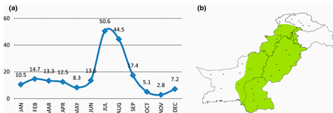
Figure 4. (a) Monthly area weighted rainfall (mm) for Pakistan; and (b) locations of meteorological stations that are available for climate data. Note that the green color shows the monsoon zone (adopted from [143]).
