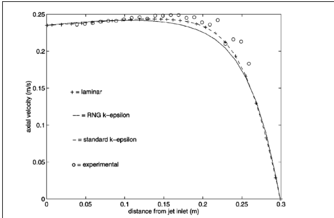
Figure 4: Comparison of LDA measurements and numerical models (cited in Posner)
