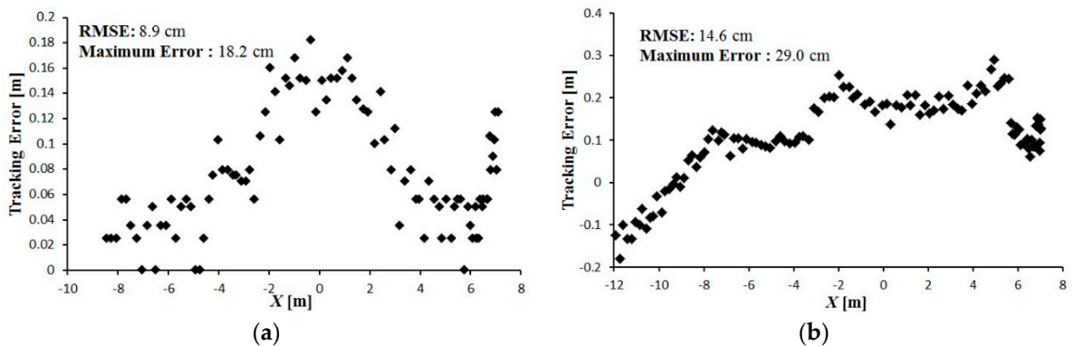
Figure 17. Tracking error between the leader and the follower trajectories during tracking on a turning path. (a) Linear tracking; (b) Parallel tracking.
