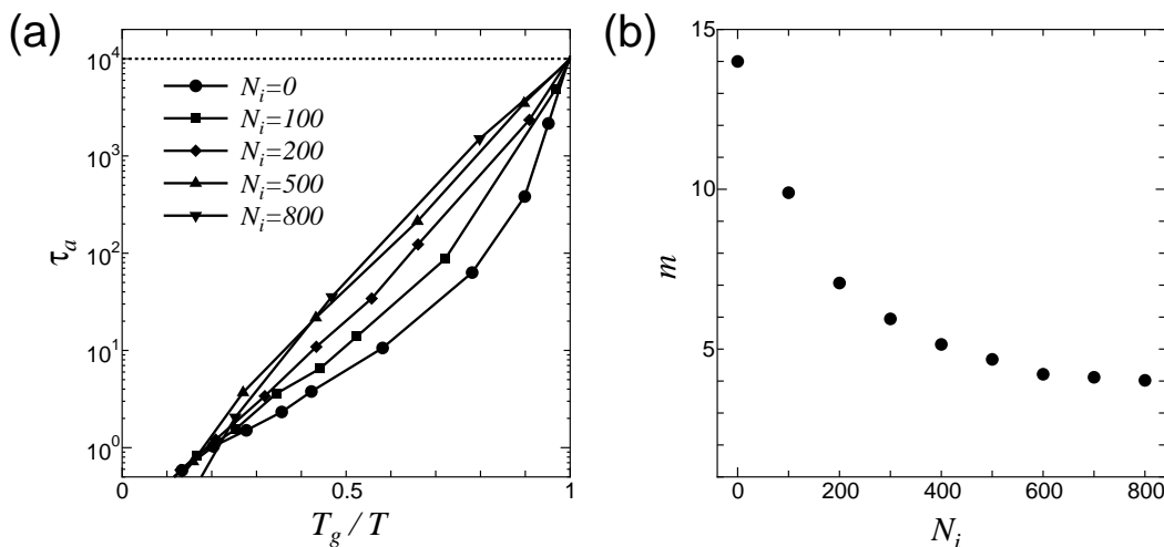
Figure 4. (a) The \alpha -relaxation time, \tau_\alpha , as a function of the inverse temperature T_g/T , for several N_i 's, N_i = 0, 100, 200, 500 and 800 . T_g is defined as the temperature at which \tau_\alpha = 10^4 . (b) N_i -dependence of the fragility index m .
