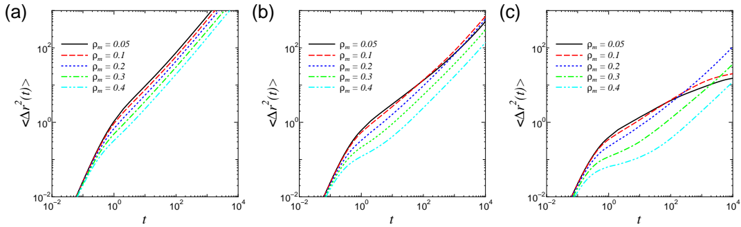
Figure 7. The \rho_m dependence of the mean square displacement, \langle \Delta r^2(t) \rangle , at the immobile particle density (a) \rho_i = 0.3 , (b) 0.43 , and (c) 0.5 of the EM systems.
