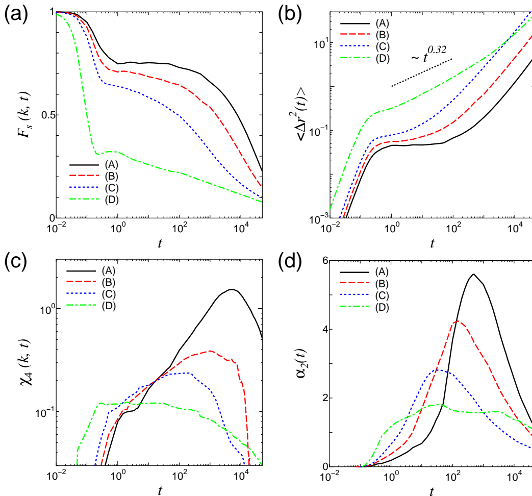
Figure 3. Various time-dependent quantities for the binary soft-core mixture generated by the EM protocol at the four state points (A) (N_i, \rho_{\text{eff}}) = (100, 1.45) , (B) (N_i, \rho_{\text{eff}}) = (300, 1.3) , (C) (N_i, \rho_{\text{eff}}) = (500, 1.15) , and (D) (N_i, \rho_{\text{eff}}) = (900, 0.7) , as denoted in Fig. 2. (a) the self-part of the intermediate scattering function F_s(k, t) with k = 2\pi , (b) the mean square displacement \langle \Delta r^2(t) \rangle , (c) the nonlinear dynamic susceptibility \chi_4(k, t) with k = 2\pi , and (d) the non-Gaussian parameter \alpha_2(t) .
