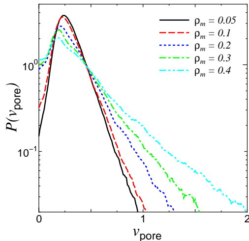
Figure 8. The pore-size distribution P(v_{\text{pore}}) for various mobile particle densities \rho_m at the fixed immobile particle density \rho_i = 0.5 of the EM systems.
