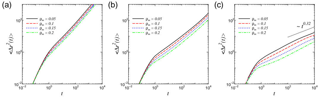
Figure 6. The \rho_m dependence of the mean square displacement, \langle \Delta r^2(t) \rangle , at the immobile particle density (a) \rho_i = 0.3 , (b) 0.43 , and (c) 0.5 of the QA systems
