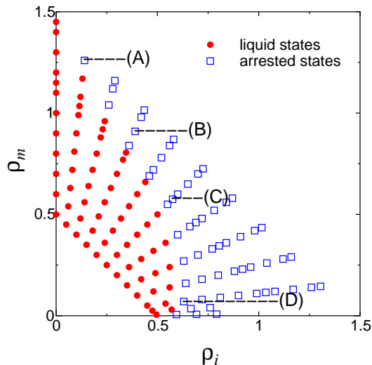
Figure 2. Dynamic phase diagram of the binary soft-core mixture generated by the EM protocol. \rho_i is the immobile (obstacle) particle density, and \rho_m is the mobile (fluid) particle density. The arrested states are defined as the points beyond which the \alpha -relaxation time \tau_\alpha exceeds 10^3 .
