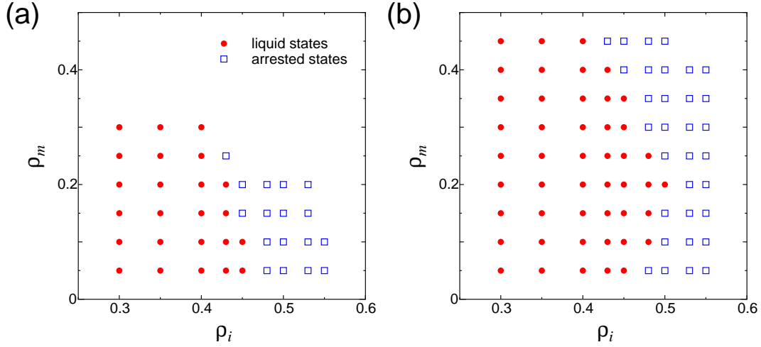
Figure 5. Dynamic phase diagram of the monodisperse hard sphere system with a random matrix generated by the two different protocols: (a) QA and (b) EM.
