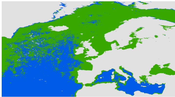
(B) Case-1 (blue) and Case-2 (green) waters around Europe
