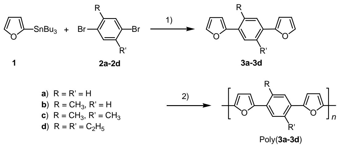
SCHEME 1. 1) [Pd(PPh 3 ) 4 ], toluene. 2) Cholesteric liquid crystal, electrochemical polymerization.
