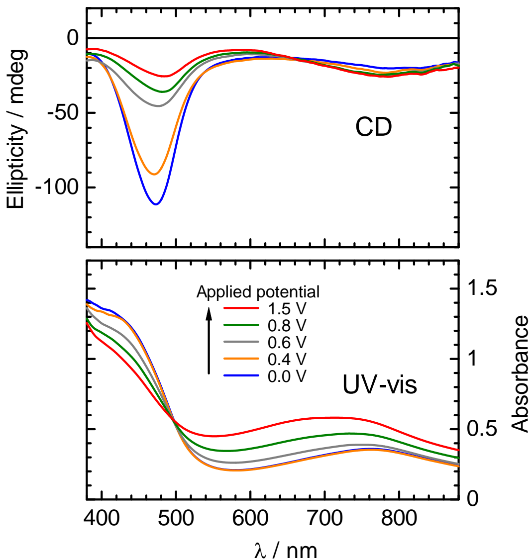
FIGURE 3. CD (top) and optical absorption (bottom) spectra of the poly(1,4-di(2-furyl)phenylene) prepared by cholesteric liquid crystal asymmetric electrochemical polymerization at various applied potentials vs. \text{Ag}/\text{Ag}^+ reference electrode during oxidation process.
