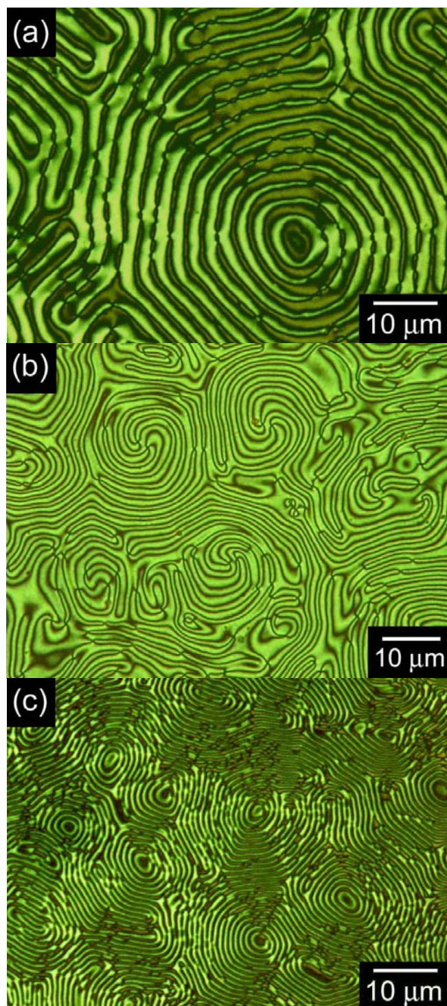
FIGURE 6 Polarizing optical microscopic images of poly(1,4-di(2-furyl)phenylene)s prepared in CLC solutions at different concentrations of the CLC inducer. (a; 4.0 wt% , b; 8.0 wt%, c; 12.0 wt%).
