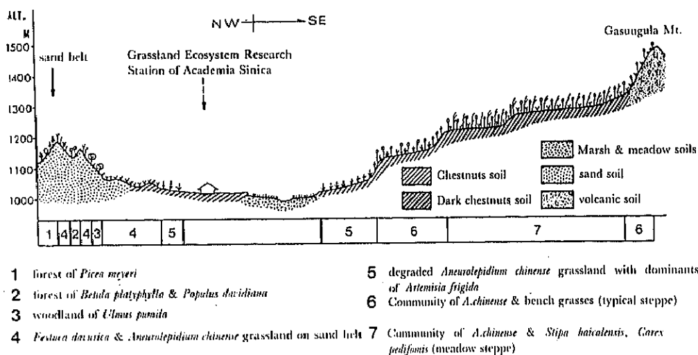
Fig. 3. A sketch map for the distribution patterns of vegetation types and its corresponding natural environments at the Bajinxile region
