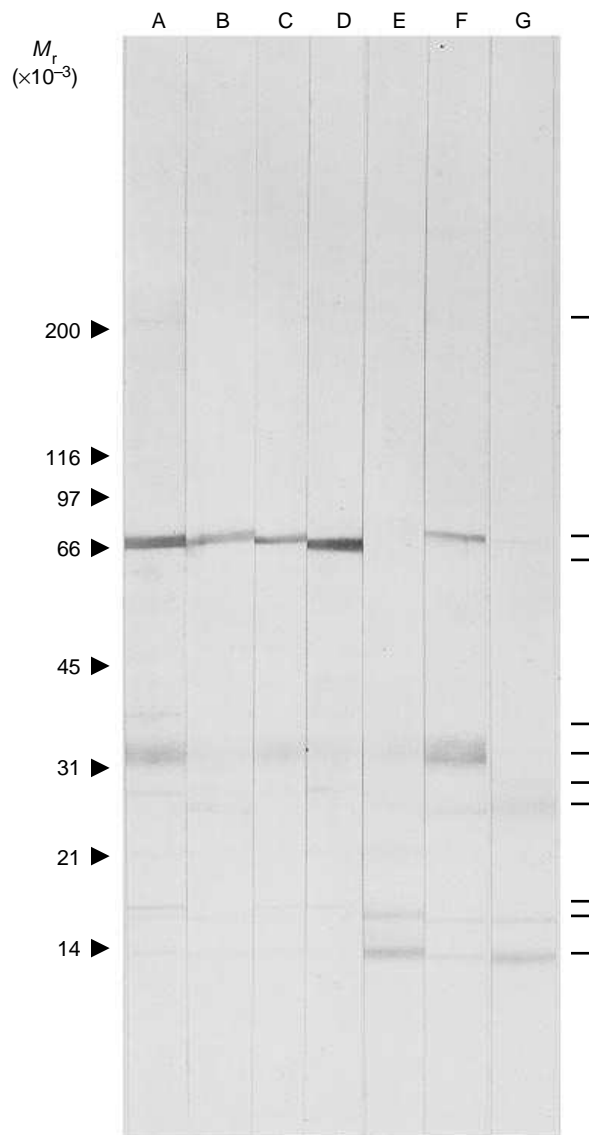
Fig. 3. Western blotting analysis of different antigen preparations probed with WTS week 8, diluted 1:1000. The antigen preparations were loaded at the same protein concentration ( 20 \mu\text{g}/\text{well} ) in the following order. (A) Male-only SWAP, (B) soluble oesophageal fraction, (C) soluble gonad preparation, (D) soluble parasite material depleted of oesophageal and gonad components (rear), (E) isolated tegumental membrane fraction, (F) female-only SWAP, (G) adult worm in vitro culture supernatant. Antigens are shown by bars.
