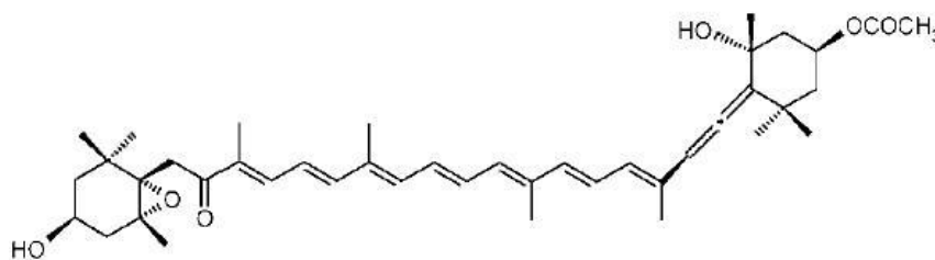
Figure 1. The structure of fucoxanthin.
