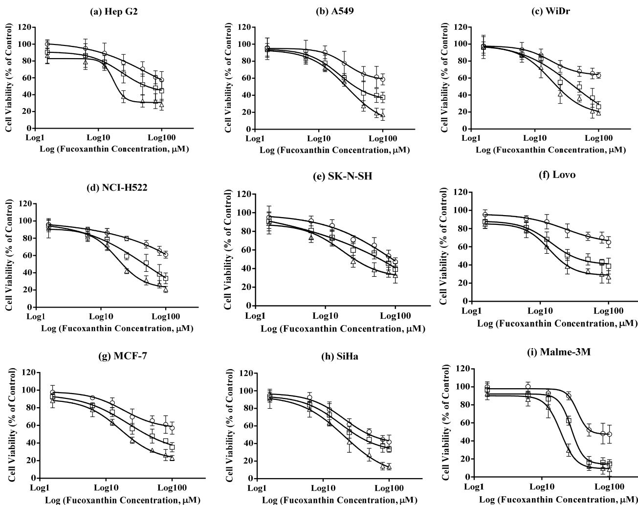
Figure 3. Inhibitory effects of pure fucoxanthin standard. All nine cancer cell lines were treated with 1.5625, 6.25, 12.5, 25, 50, 80, 100 \mu\text{M} fucoxanthin. Inhibitory effects were determined after treatment at 24 h ( \circ ), 48 h ( \square ) and 72 h ( \Delta ). Data are expressed as mean \pm standard errors ( n = 6 ). (a) In Hep G2 cell line; (b) in A549 cell line; (c) in WiDr cell line; (d) in NCI-H522 cell line; (e) in SK-N-SH cell line; (f) in Lovo cell line; (g) in MCF-7 cell line; (h) in SiHa cell line; (i) in Malme-3M cell line.
