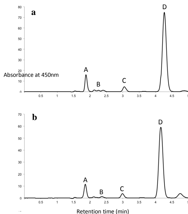
Figure 2. HPLC chromatograms of (a) the 1st NZ U. pinnatifida extract; (b) the 2nd NZ U. pinnatifida extract. Peaks in chromatograms: (A) trans -fucoxanthin; (B) cis -fucoxanthin; (C) unidentified peak; (D) canthaxanthin (internal standard).
