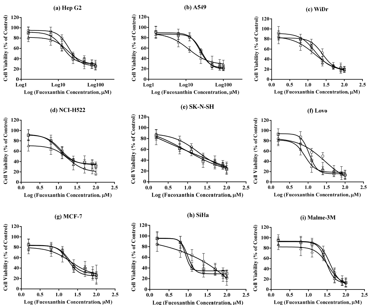
Figure 4. Inhibitory effects of three extracts from NZ U. pinnatifida (containing 0.2 ( \Delta ), 43.5 ( \square ) and 60.8% ( \circ ) fucoxanthin, respectively) on nine cancer cell lines. Data are expressed as mean \pm standard errors (n = 6). (a) In Hep G2 cell line; (b) in A549 cell line; (c) in WiDr cell line; (d) in NCI-H522 cell line; (e) in SK-N-SH cell line; (f) in Lovo cell line; (g) in MCF-7 cell line; (h) in SiHa cell line; (i) in Malme-3M cell line.
