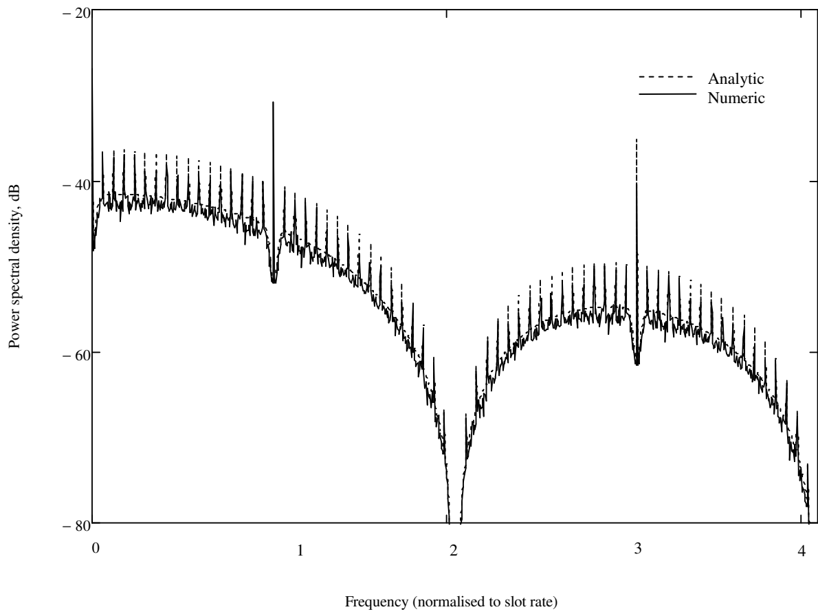
Fig. 2 Power spectral density of SPPM with n=17 and t_p = \frac{t_s}{2}
