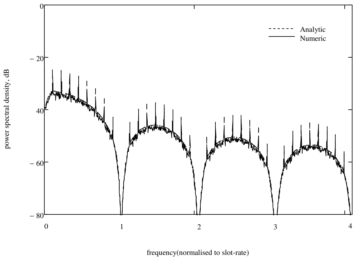
Fig. 1 Power spectral density of SPPM with n = 9 and t_p = t_s
