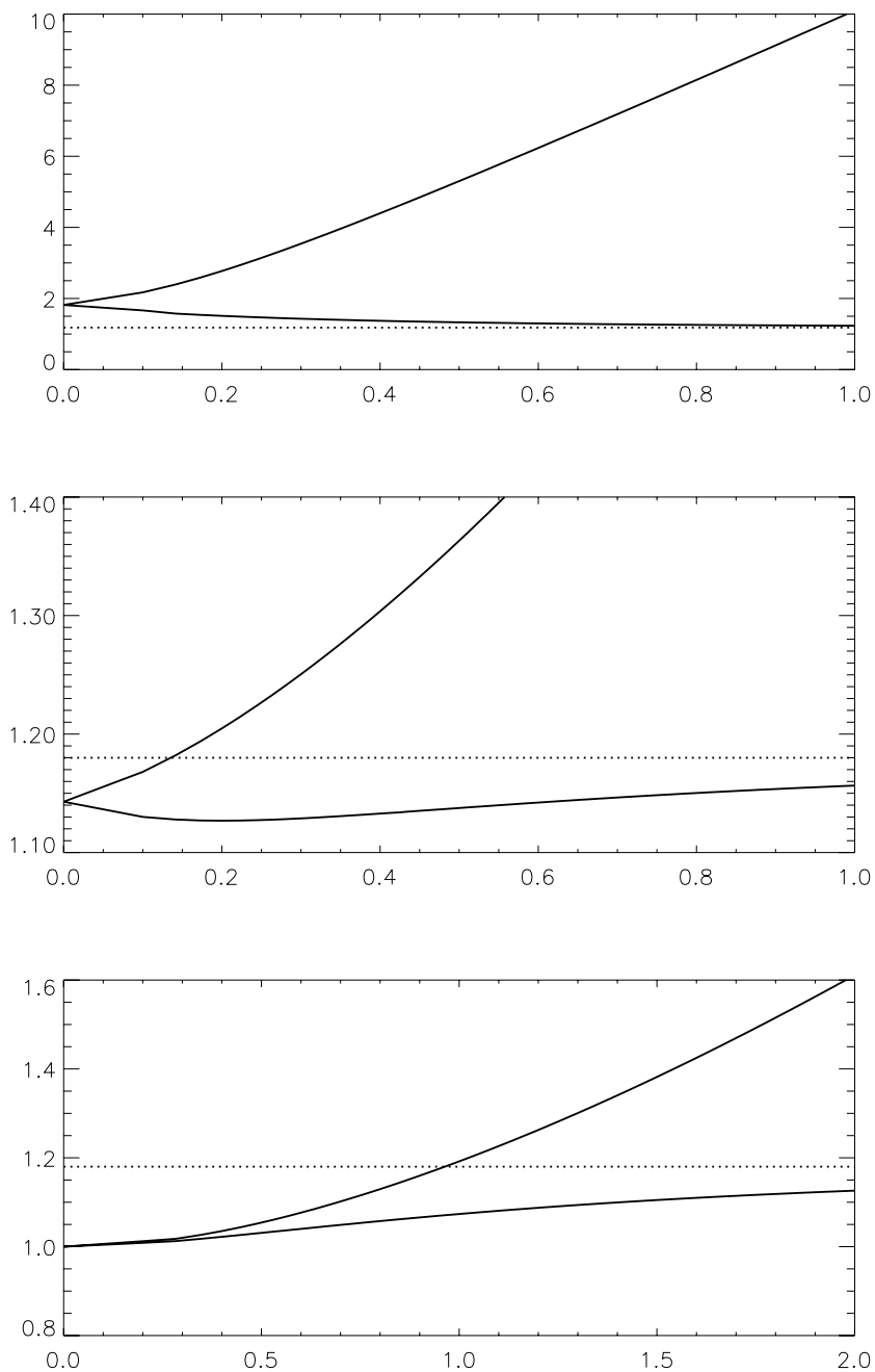
Figure 3. The dependences of the boundaries of the instability interval with respect to the wavenumber, k_1 and k_2 , on a . The upper panel corresponds to b = 0.1 , the middle panel to b = 0.75 , and the lower panel to b = 1.5 . The dependences of k_1 and k_2 on a are qualitatively the same as in the upper panel when b^2 < 1/3 , as in the middle panel when 1/3 < b^2 < 1 , and as in the lower panel when b > 1 . The horizontal dotted lines are the asymptotes for k_1(a) as a \rightarrow \infty .
