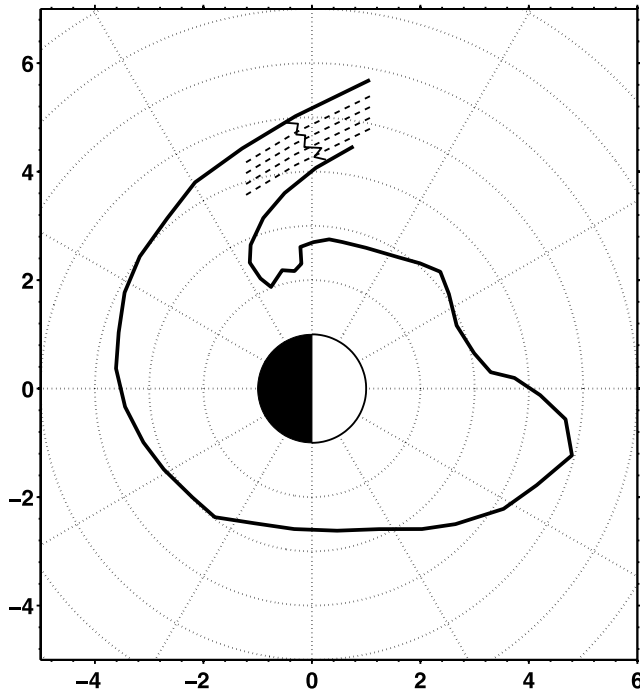
Figure 1. Schematic diagram of the plasmopause location and attached plume structure wrapping around during storm time condition, reproduced from EUV measurement at 0939 UT 10 June 2001 [Spasojević et al. , 2003, Figure 12c]. Wiggly solid line illustrates the density variation inside the plume, and four dashed lines represent plasma density contour.
