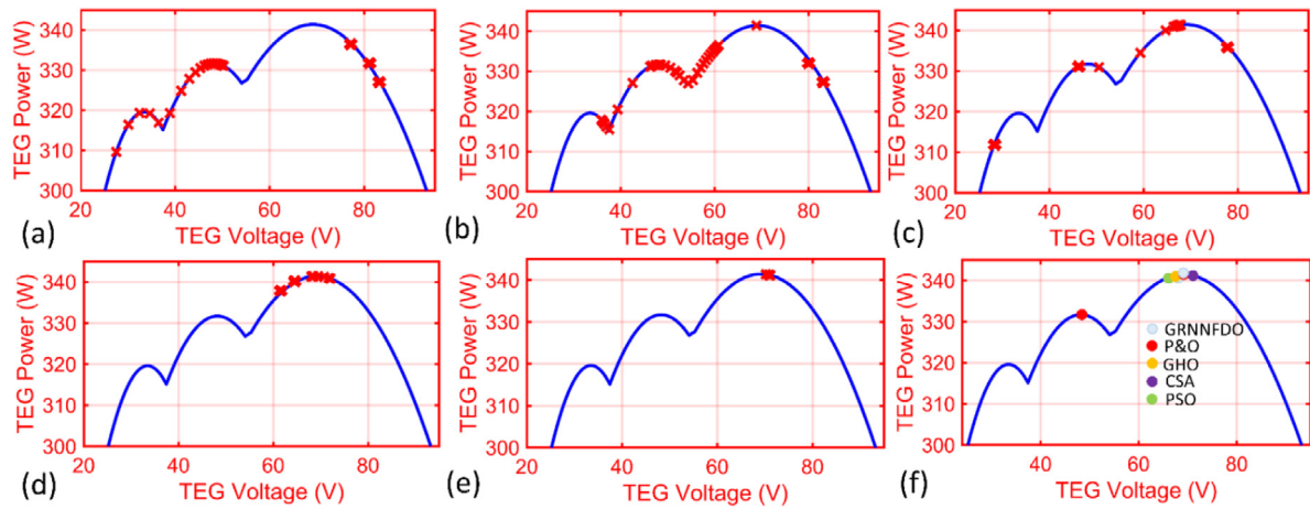
Fig. 13. Case study 2: GRNNFDO GMPP tracing under NUTD.
