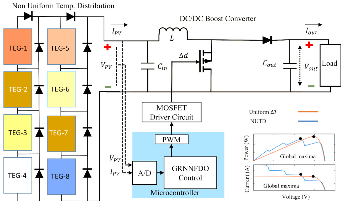
Fig. 1. TEG modules linked with DC – DC Boost converter through proposed GRNNFDO control.
