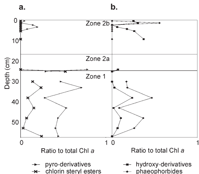
Fig. 7. Depth profiles of a. pyro-derivatives and CSEs, and b. 13^2 -hydroxy-derivatives and Pheids relative to the total Chl a signal in the Progress Lake sediment.
