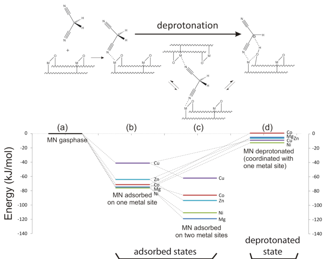
Figure 5. Schematic representation of adsorption and subsequent deprotonation reaction of malononitrile (MN), and corresponding energy profiles for different M 2 dobdc materials. MN can be adsorbed on one (b) or two adjacent metal sites (c). Note that the deprotonation of MN, adsorbed at two metal sites, can only occur if one nitrile-metal coordination is released (d).
