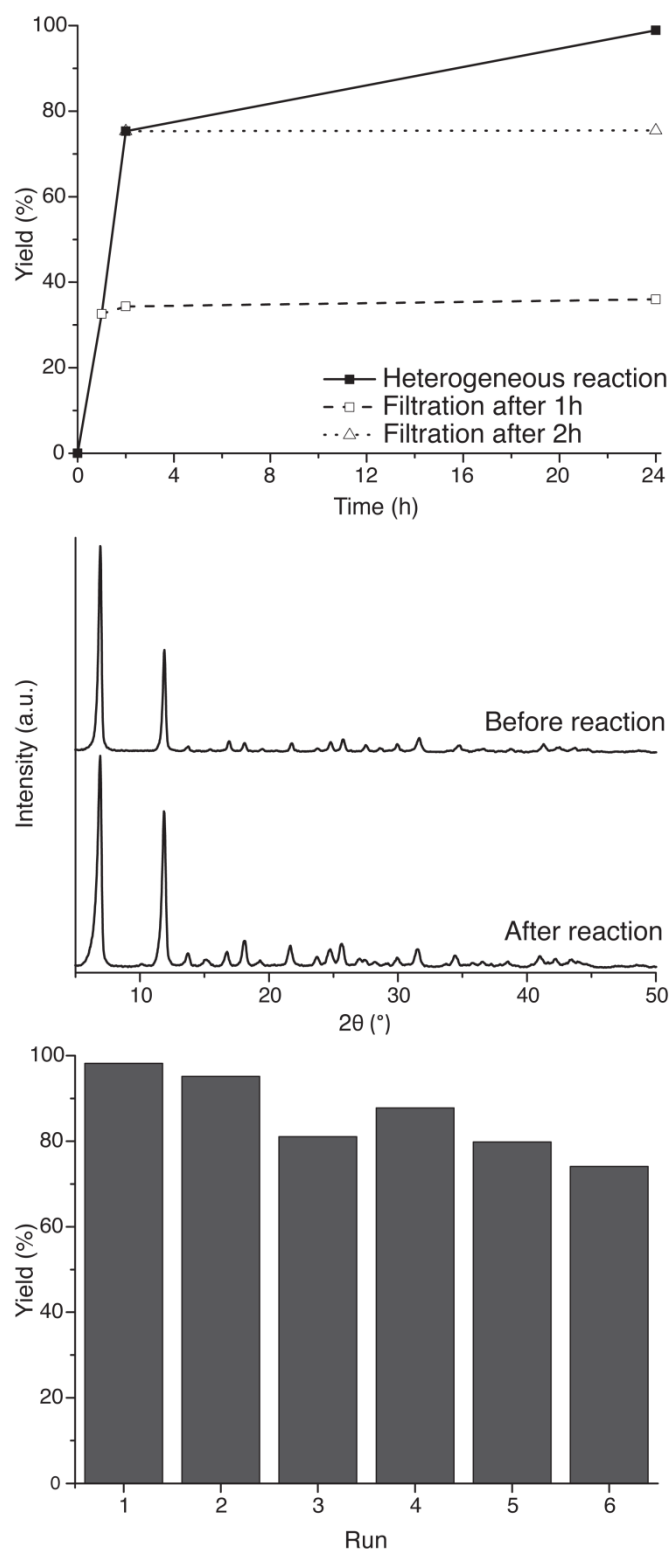
Figure 3. Hot filtration test for \text{Ni}_2\text{dobdc} in the Knoevenagel condensation of malononitrile with benzaldehyde (top), PXRD diffraction patterns before and after reaction (middle) and product yield in consecutive runs with the catalyst (bottom).
