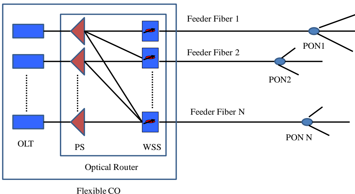
Figure 3. Flexible CO design to share OLTs with PON segments dynamically.
