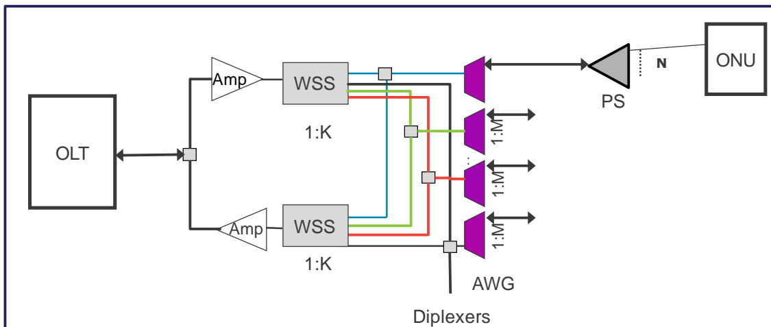
Figure 8: Wavelength Switched TWDM-PON architecture
