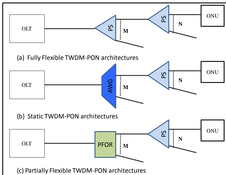
Figure 4: Different variants of TWDM-PON based on the degree of flexibility, where remote node 2 is always a power splitter (PS).
