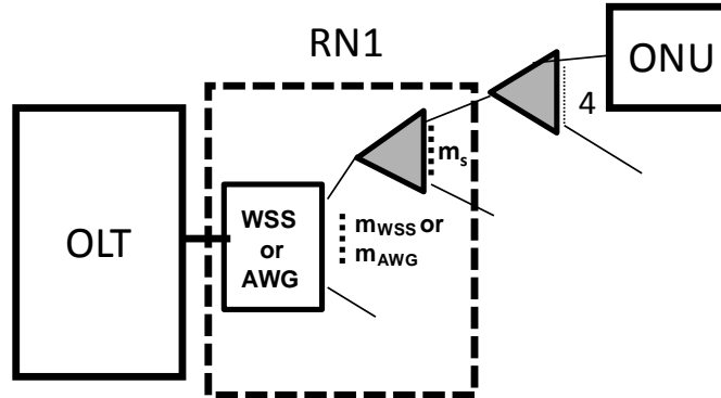
Figure 5: TWDM-PON flavour based on AWG and power splitters considered for evaluation
