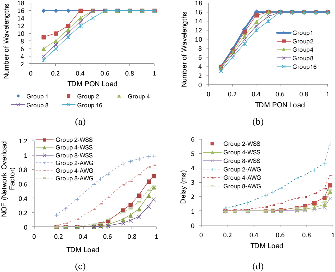
Figure 7: Illustrates the performance for five TWDM-PON variants with a different degree of flexibility in RN1 for highly bursty traffic in (a) Average number of wavelengths required in function of the TDM-PON or RN2 load in an AWG based RN1, (b) Average number of wavelengths required in function of the offered TDM-PON or RN2 load in a WSS based RN1, (c) Probability of an overloaded situation in a TDM-PON for varying load for WSS and AWG based configuration, (d) Delay vs. load for TWDM-PON variants with a different degree of flexibility in WSS and AWG based RN1 configuration
