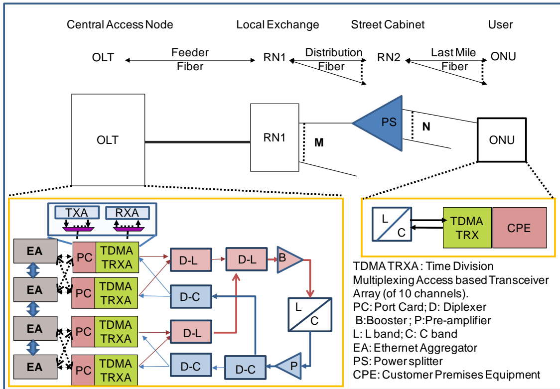
Figure 2: General TWDM-PON architecture, consisting of two remote nodes
