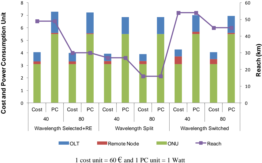
Figure 9: Cost, Power Consumption and Reach comparison of various TWDM-PON variants
