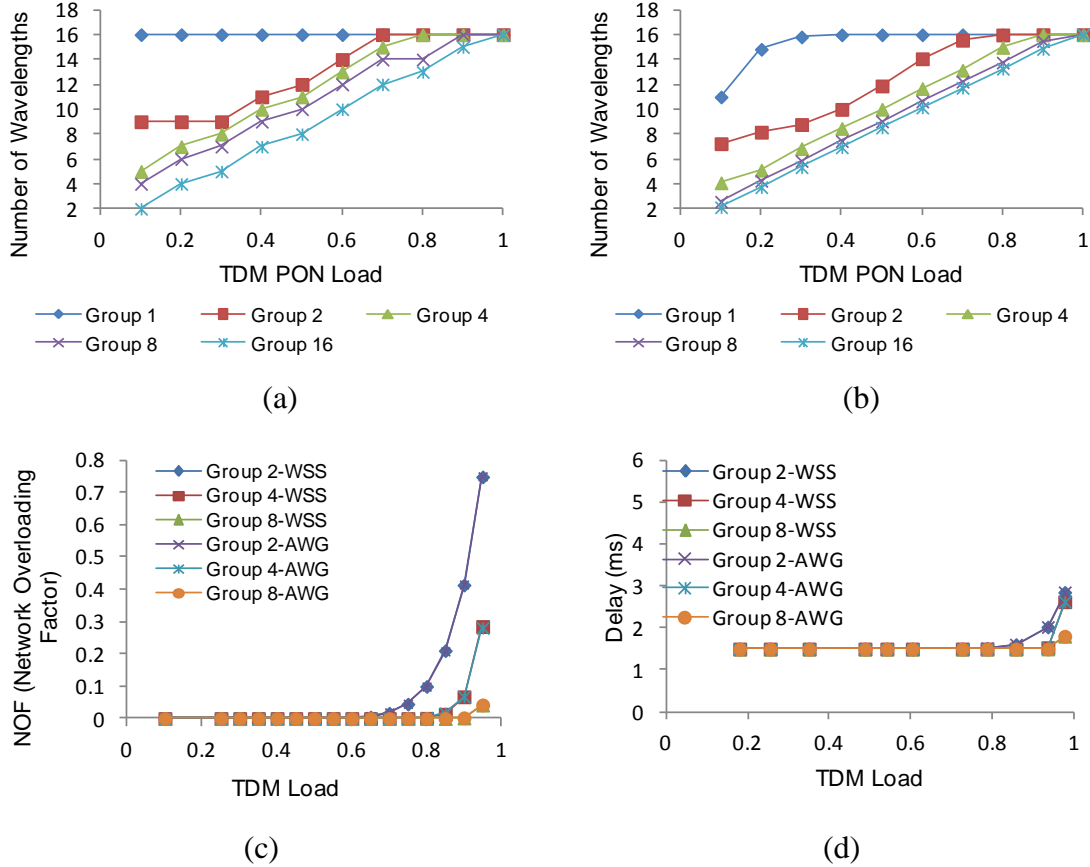
Figure 6: Illustrates the performance for five TWDM-PON variants with a different degree of flexibility in RN1 for less bursty traffic in (a) Average number of wavelengths required in function of the TDM-PON or RN2 load in an AWG based RN1, (b) Average number of wavelengths required in function of the offered TDM-PON or RN2 load in a WSS based RN1 (c) Probability of an overloaded situation in a TDM-PON for varying load for WSS and AWG based configuration, (d) Delay vs. load for TWDM-PON variants with a different degree of flexibility in WSS and AWG based RN1 configuration
