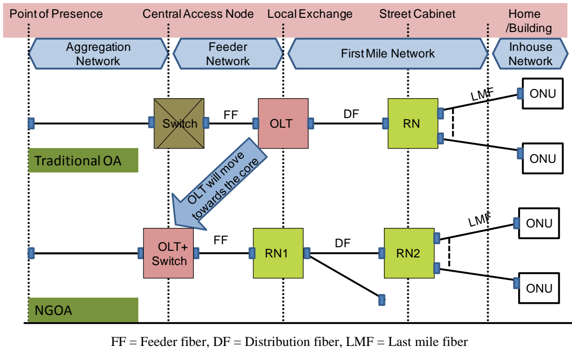
Figure 1: Difference between traditional optical access (OA) and next-generation optical access (NGOA) scenarios
