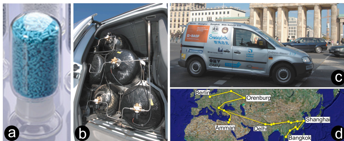
Figure 18 – EcoFuel Asia Tour 2007 - Berlin to Bangkok: 32 000 km with Basolite C300 in tank. (a) Basolite C300 (HKUST-1); (b) MOF-enhanced fuel tanks with CH 4 ; (c) Volkswagen Caddy EcoFuel prototype car; (d) journey map. (Adapted with permission from ref. 193.)
