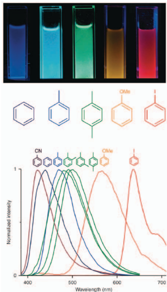
Figure 14 - (top) Luminescence of the powdered [\text{Zn}_2(\text{bdc})_2(\text{dpNDI})]_n material suspended in aromatic VOC liquids, with the corresponding structures below, after excitation at 365 nm using a commercial ultraviolet lamp. (bottom) Collected normalized spectra of the [\text{Zn}_2(\text{bdc})_2(\text{dpNDI})]_n > \text{VOC} compounds excited at 370 nm. (Adapted with permission from ref. 191. Copyright 2011 Macmillan Publishers Limited.)
