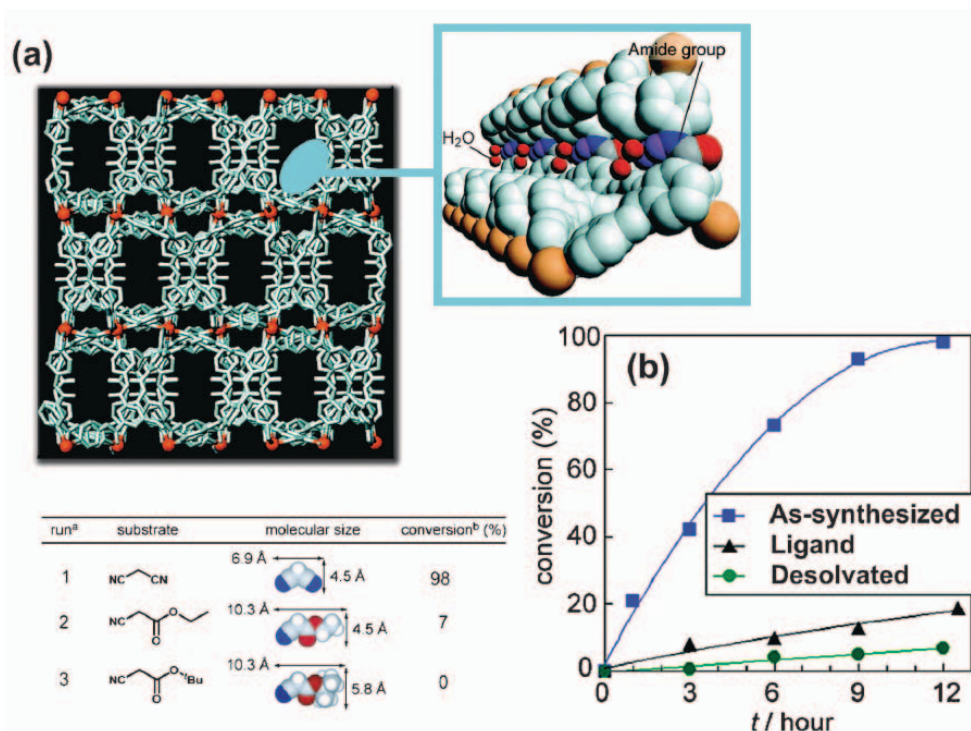
Figure 12 - (a) Crystal structure of \{[\text{Cd}(4\text{-btapa})_2(\text{NO}_3)_2] \cdot 6\text{H}_2\text{O} \cdot 2\text{DMF}\}_n emphasizing the zigzag channels present in the structure. (top right) View of the ordered amide groups decorating the surface of the channels and interacting with water molecules via hydrogen bonds. Cd atoms = light brown, O atoms = red, N atoms = blue, C atoms = gray and H atoms = purple. (b) Conversion for the Knoevenagel condensation reaction of benzaldehyde with malononitrile catalyzed by the as-synthesized (blue squares) and desolvated (green circles) materials and organic ligand (black triangles). (bottom left) Table summarizing the results of the Knoevenagel condensation reaction for the various substrates. (Adapted with permission from ref. 170. Copyright 2007 American Chemical Society.)
