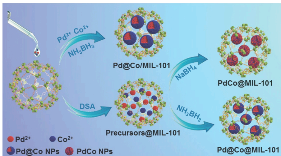
Figure 13 - Schematic representation of the preparation of the \text{Pd@Co/MIL-101} , \text{PdCo@MIL-101} and \text{Pd@Co@MIL-101} catalysts using different synthetic methodologies and reducing agents. (Reprinted with permission from ref. 177. Copyright 2015 Wiley-VCH.)
