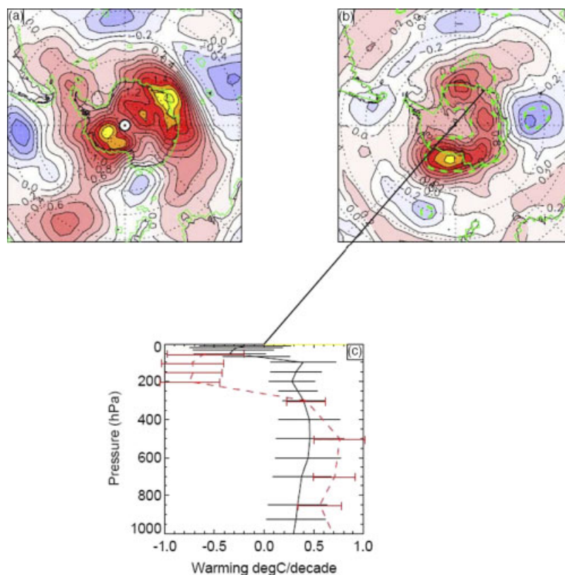
Figure 3. (a) The warming in June in ERA-40 at 500 hPa between 1979 and 2001. The maximum warming is greater in ERA-40 than in our climate model runs and the radiosonde ascents. (b) The warming in June observed between the two runs of HadAM3, the first with a 0.5 optical depth PSC layer at 100 hPa polewards of 80°S and the second with a similar layer extending to 70°S. The area of significant change at the 95% level (calculated using the student's t -test) is enclosed within the dashed green contour. Assuming the two runs represent conditions in 1980 and 2000, the warming between the runs has been divided by two to give a decadal change. (c) The observed vertical profile of the warming in June at Syowa from radiosonde data (red dashed) and from an average of an area around Syowa (65–75°S, 0–45°E) in the model runs (black).
