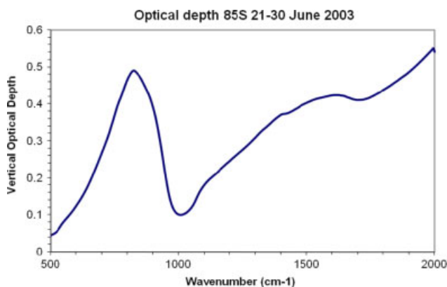
Figure 2. The mean optical depth spectrum for the last 10 days of June 2003 based on the model of Höpfner et al. (2006) using ECMWF analyses. The spectrum is dominated by absorption due to ice PSCs.
