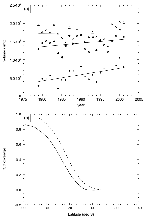
Figure 1. (a) The volume of air above the Antarctic where the ERA-40 temperature is below the ice point. This represents the volume of air potentially containing ice PSCs. The crosses are for June, the stars for July and the triangles for August. (b) The zonal average of the potential coverage of an ice PSC cloud for June at 100 hPa in 1979 (solid) and 2001 (dashed) similarly calculated.
