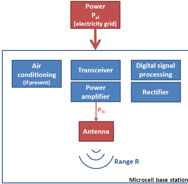
Figure 1. Block diagram of microcell base station equipment.
