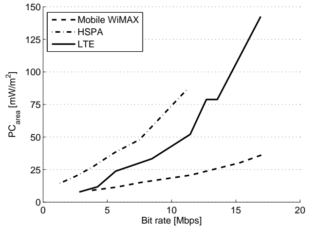
Figure 2. Energy efficiency of a microcell base station for different bit rates in 5 MHz channel.
