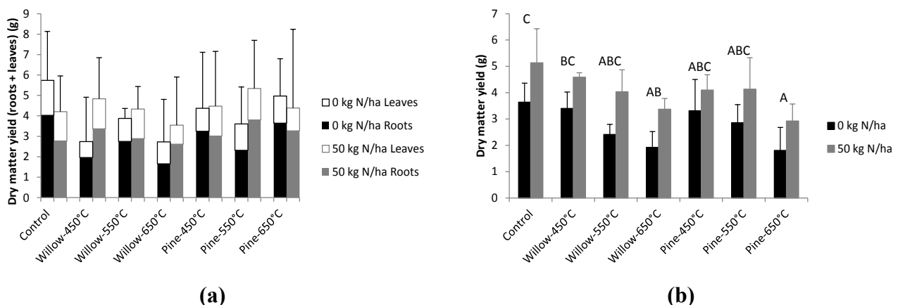
Figure 7. (a) Radish and (b) spring barley dry matter yield (per pot) in the control and biochar-amended treatments at two fertilizer doses (0 and 50 kg N ha -1 ) in the DTU pot trial; error bars indicate \pm 1 standard deviation ( n = 4 ); for (a) no significant differences were found; for (b) treatments with different letters differ significantly ( P < 0.05 ) according to a Scheffé-test (one letter per biochar treatment due to no interaction between factors biochar type and fertilizer dose).
