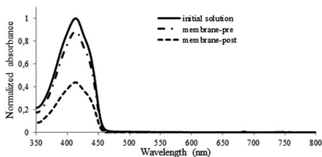
Figure 5. UV spectra of DPBF/THF solutions. Initial DPBF/THF solution and after 30 min of irradiation membrane-pre and membrane-post in THF.
