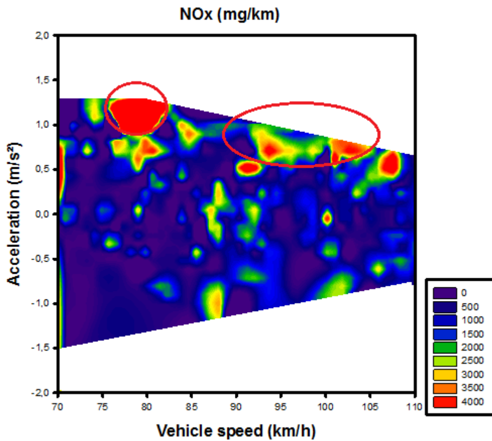
Figure 15: Contour plot of tailpipe NOx emissions in mg/km of vehicle 4 (CADC)
