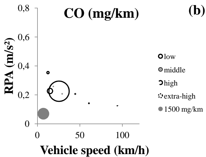
Figure 9: Bubble chart of tailpipe NO x emissions (a) and CO emissions (b) of vehicle 3 (WLTC)
