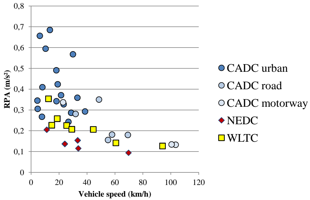
Figure 1: RPA vs. vehicle speed for NEDC, CADC and WLTC
