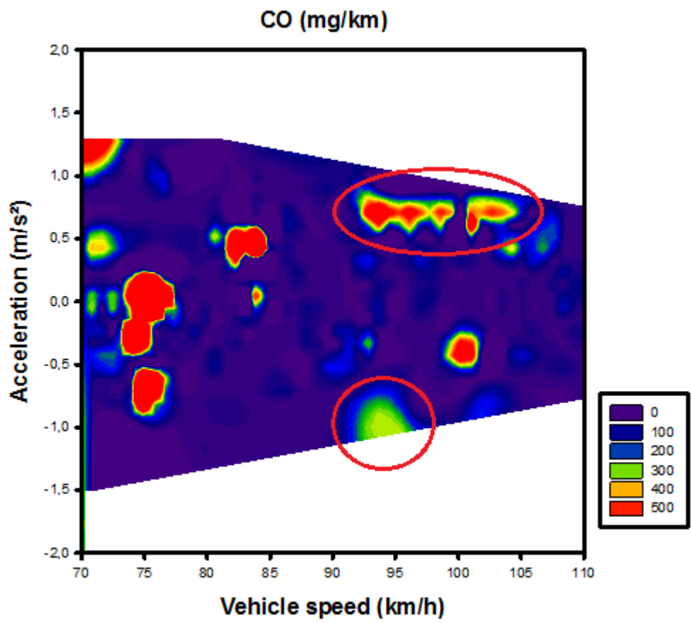
Figure 14: Contour plot of tailpipe CO emissions in mg/km of vehicle 3 (CADC)
