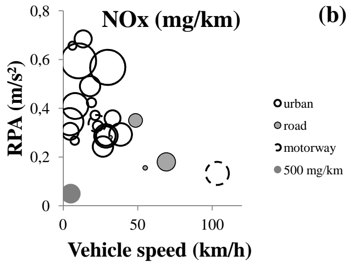
Figure 12: Bubble chart of tailpipe NO x emissions of vehicle 4 (WLTC (a) and CADC (b)).
