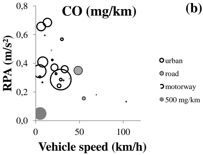
Figure 11: Bubble chart of tailpipe NO x emissions (a) and CO emissions (b) of vehicle 3 (CADC)
