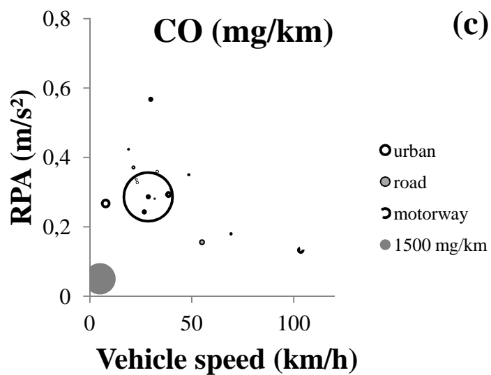
Figure 8: Bubble chart of tailpipe CO emissions of vehicle 2 (WLTC (a), NEDC (b) and CADC (c)).
