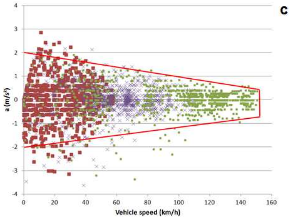
Figure 3: Acceleration vs. vehicle speed for NEDC (a), WLTC (b) and CADC (c)
