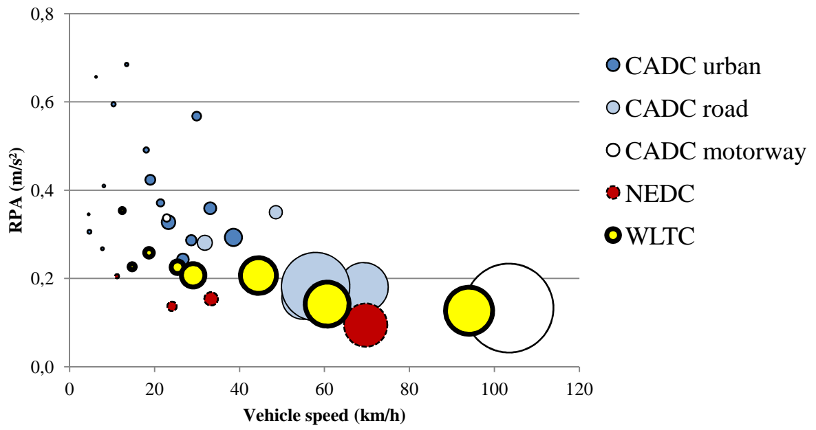
Figure 2: Bubble chart of the distance of the trips for NEDC, CADC and WLTC
