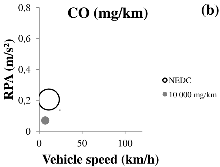
Figure 10: Bubble chart of tailpipe NO x emissions (a) and CO emissions (b) of vehicle 3 (NEDC)
