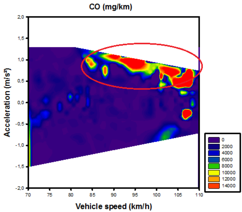
Figure 16: Contour plot of tailpipe CO emissions in mg/km of vehicle 5 (CAD/C)
