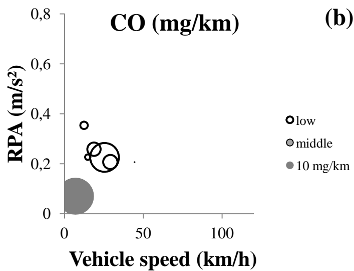
Figure 7: Bubble chart of tailpipe CO emissions of vehicle 4 (WLTC (a) and phase 1 and 2 of WLTC with hot start (b))
