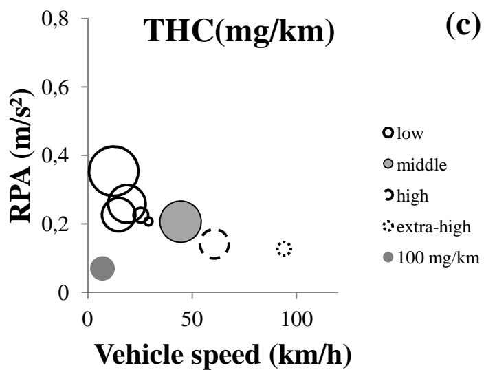
Figure 5: Bubble chart of tailpipe NO x emissions (a), CO emissions (b) and THC emissions (c) of vehicle 1 (cold-start WLTC)
