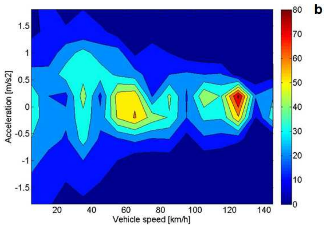
Figure 4: contourplot of acceleration vs. vehicle speed for WLTC (a) and CADC (b)
