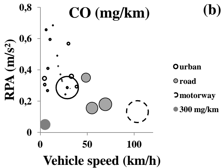
Figure 17: Bubble chart of tailpipe CO emissions of vehicle 5 (WLTC (a) and CADC (b)).
