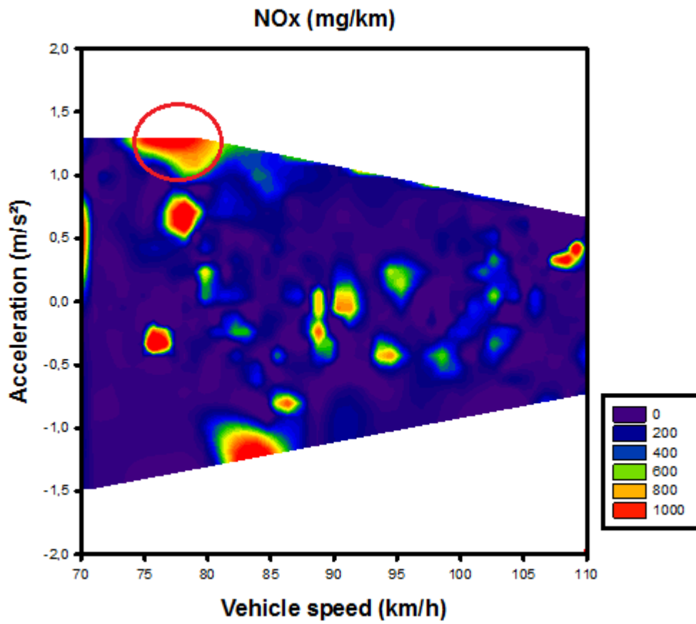
Figure 13: Contour plot of tailpipe NOx emissions in mg/km of vehicle 3 (CADC)
