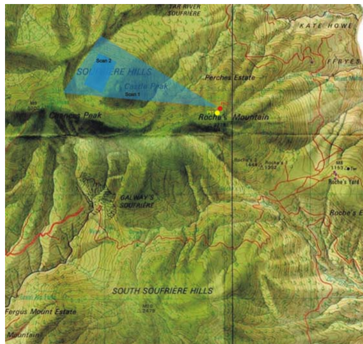
Figure 2 Location of laser scanner (red) and backsight (yellow) positions showing general directions of scans (blue).
