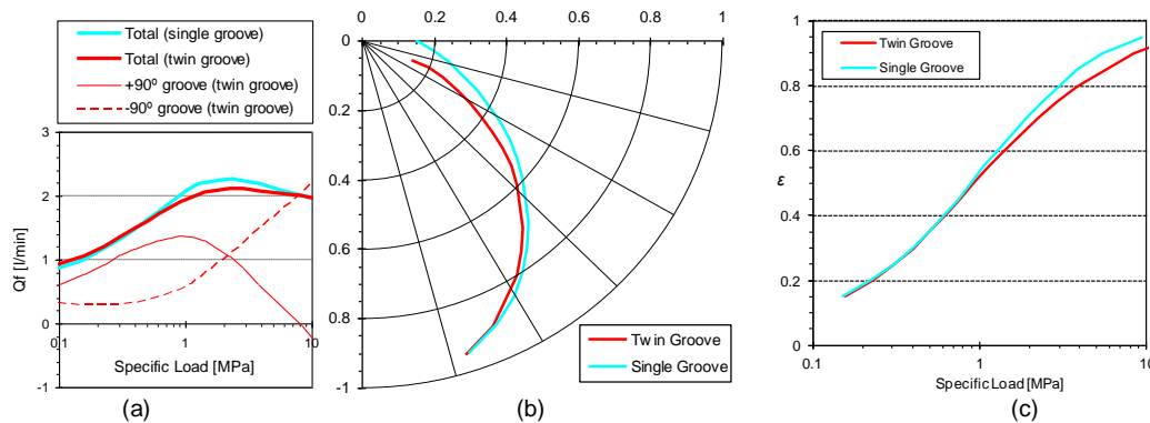
Fig. 21 - Influence of the number of grooves on (a) the lubricant flow rates and (b) on shaft locus and (c) on eccentricity ratio.
