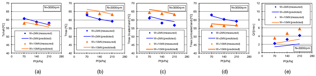
Fig. 10 - Comparison between theory and experiment, for several loads and feeding pressures, of (a) Shaft surface temperature, (b) maximum bush temperature, (c) maximum bush temperature at the loaded (lower) land, (d) maximum bush temperature at the unloaded (upper) land of the bearing and (e) flow rate. [24]
