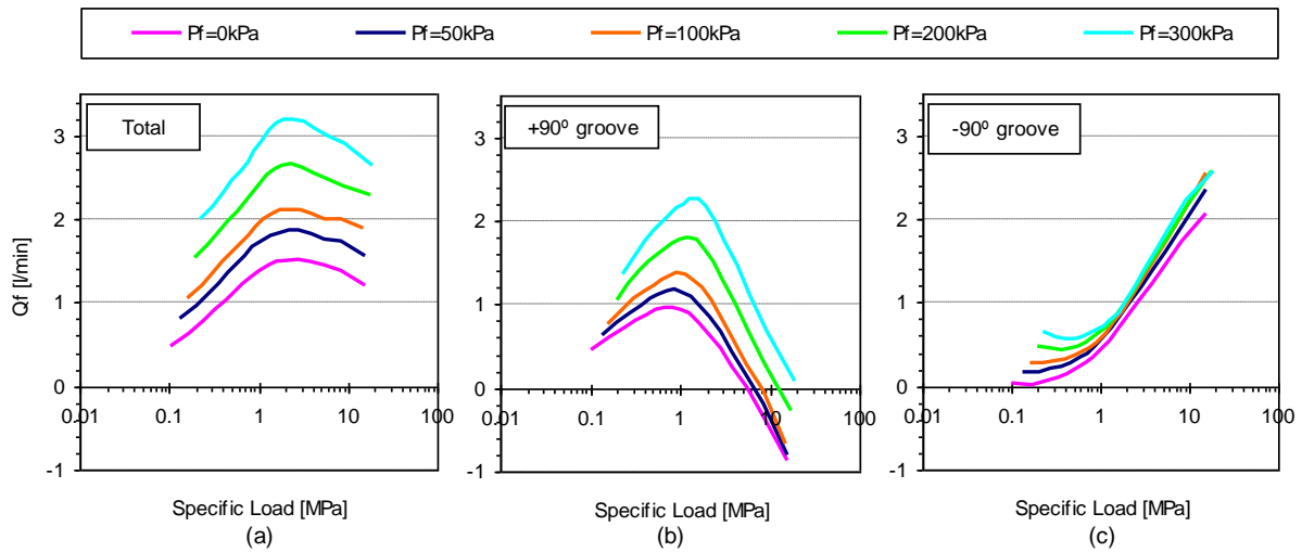
Fig. 11- Influence of specific load and lubricant feeding pressure on (a) total flow rate, (b)+90° groove flow rate and (c) -90° groove flow rate (N=3000rpm).
