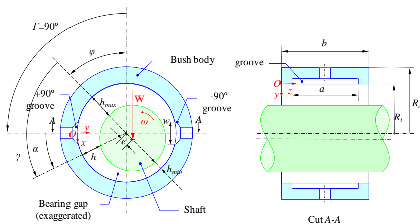
Fig. 1 - Outline of the bearing geometry
