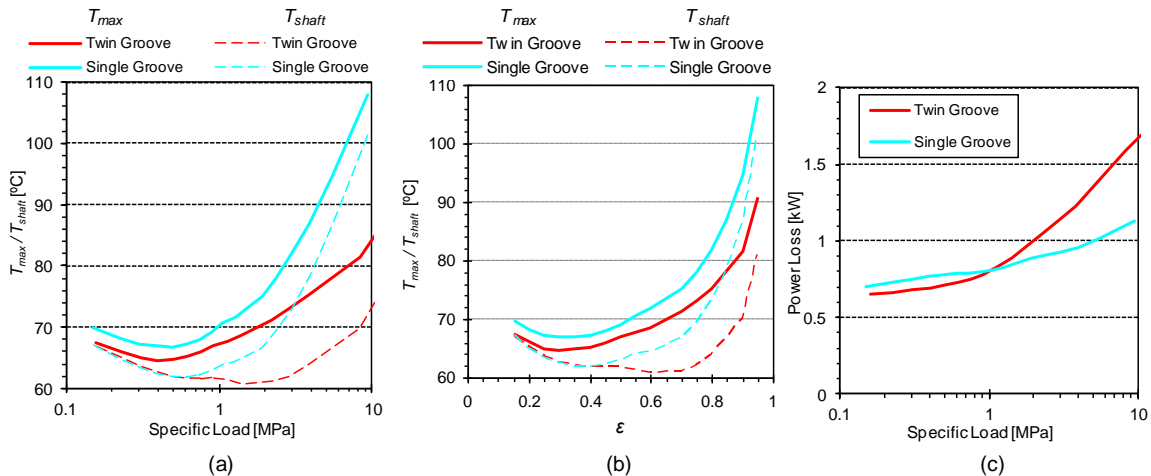
Fig. 23 - Influence of the number of grooves on the maximum bush temperature and the shaft surface temperature as a function of (a) specific load and (b) eccentricity ratio. (c) Influence of the number of grooves in power loss.
