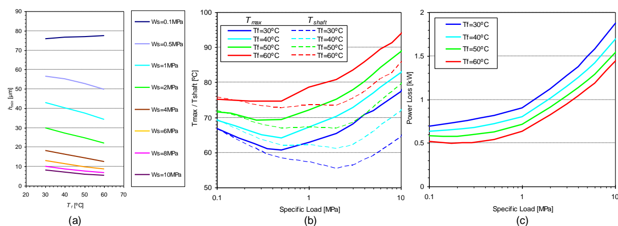
Fig. 15 – (a) Influence of feeding temperature on (a) minimum film thickness, (b) maximum bush temperature and shaft surface temperature and (c) power loss as a function of specific load ( N=3000\text{rpm} ).
