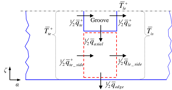
Fig. 6 - Outline of the thermal balance carried out to determine the average inlet section temperature, \bar{T}_{is} , which incorporates the influence of the groove length ratio, a/b
