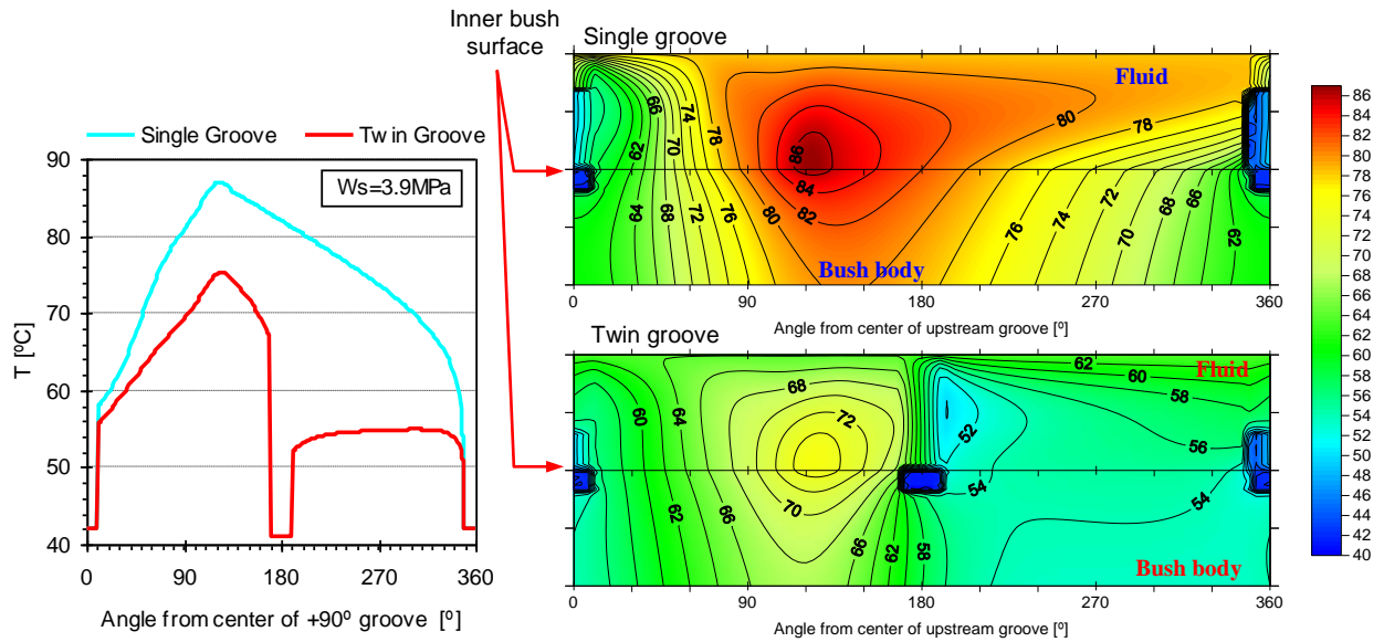
Fig. 22 - Influence of the number of grooves on (a) the temperature profile at the midplane of the inner bush surface and (b) the midplane temperature field of the fluid domain and of the bush body domain ( W_s=3.9\text{MPa} ).
