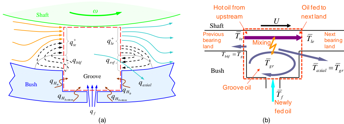
Fig. 5 – (a) Heat fluxes across the boundaries of the groove region in the presence of back flow upstream and reverse flow downstream of the groove; (b) Outline of the thermal mixing model within the groove region.
