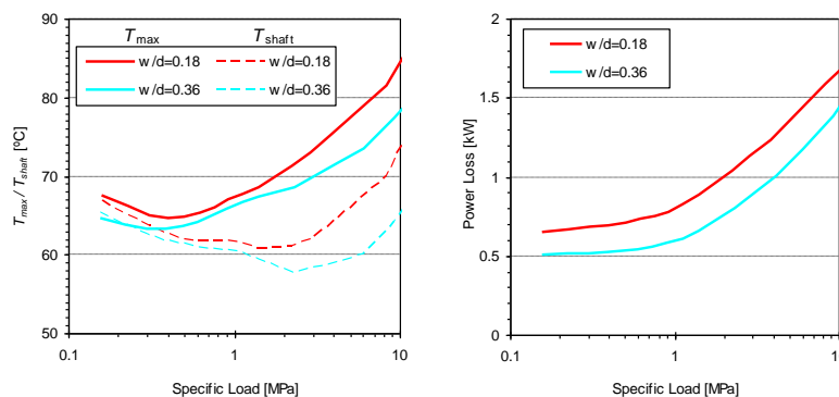
Fig. 20 - Influence of groove width ratio on (a) maximum bush and shaft surface temperature and (b) on power loss.
