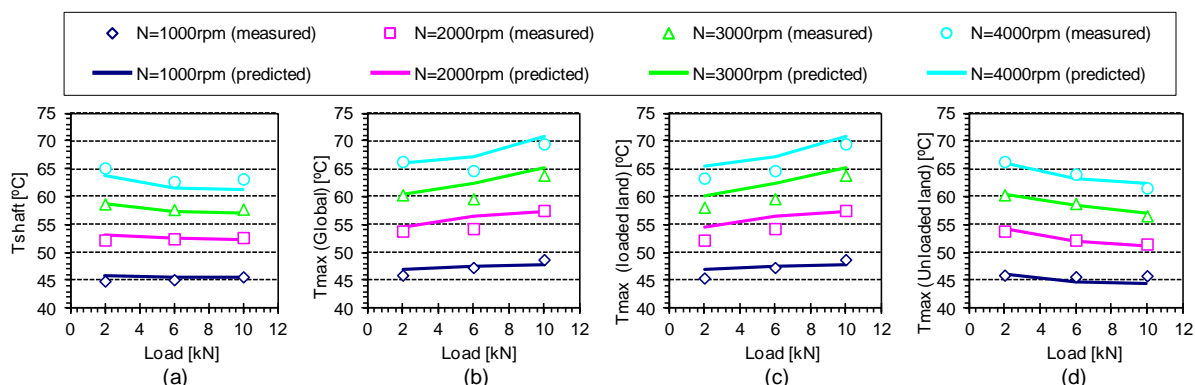
Fig. 9 - Comparison between theory and experiment, for several loads and shaft speeds, of (a) Shaft surface temperature, (b) maximum bush temperature, (c) maximum bush temperature at the loaded (lower) land and (d) maximum bush temperature at the unloaded (upper) land of the bearing (Pf=140kPa);[39]
