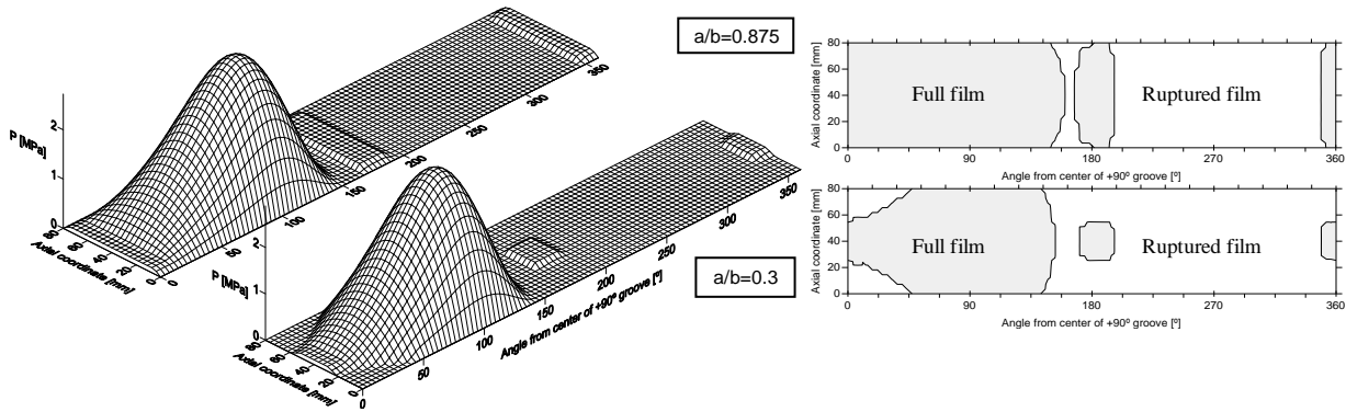
Fig. 17 - Influence of groove length ratio on (a) the hydrodynamic pressure field and (b) extension of full film and ruptured film regions ( W_s=1.1\text{MPa} )
