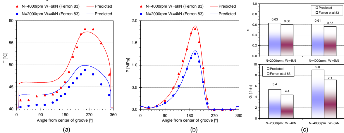
Fig. 7 – Comparison between the present analysis and experimental data [38] under two different conditions, for (a) inner bush surface temperature profile (b) pressure profile at the midplane of the bearing and (c) eccentricity ratio and flow rate.
