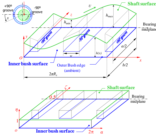
Fig. 2 – Unwrapped dimensional and non-dimensional (normalized) fluid domain
