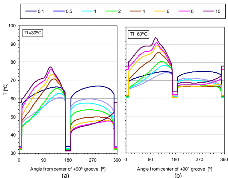
Fig. 16 - Temperature profile at the midplane of the inner bush surface for several specific loads and (a) T_f=30^\circ and (b) T_f=60^\circ\text{C}
