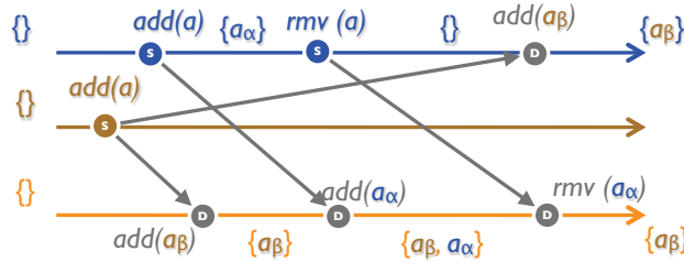
Figure 11: Observed-Remove Set (op-based)
