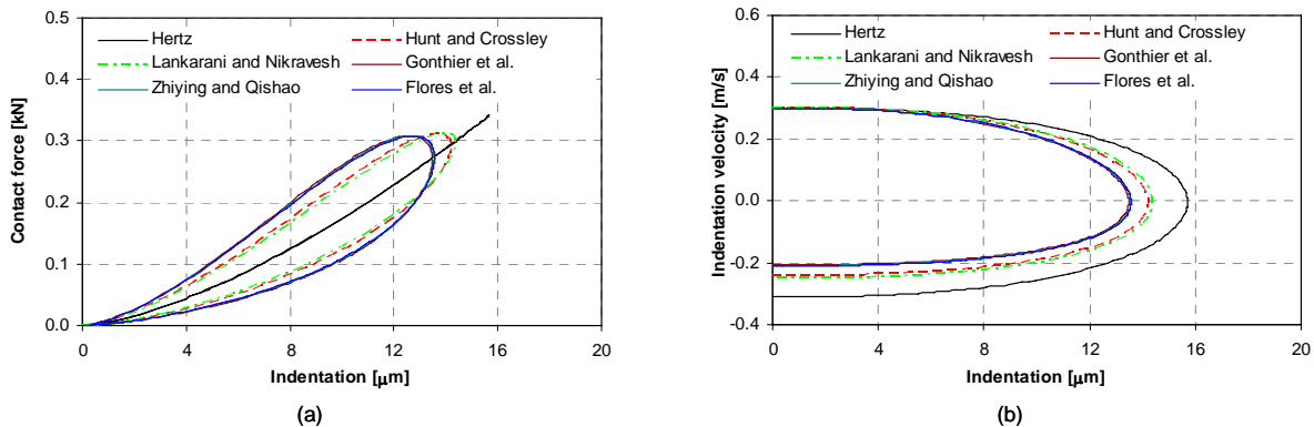
Fig. 6 Externally colliding spheres modeled by Hertz, Hunt and Crossley, Lankarani and Nikravesh, Gonthier et al., Zhiying and Qishao, and Flores et al. contact force models: (a) Force-indentation relation; (b) Phase portrait.
