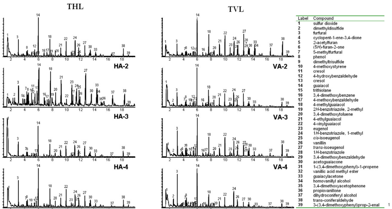
Fig. 6. Py-GC/MS of calcium liginosulfonate during incubation with Trametes hirsuta laccase (THL) and Trametes villosa laccase (TVL) in the presence of HBT.
