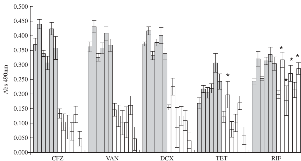
Figure 3. Mean reduction of cellular activity, measured by XTT, after 3 h of exposure to the antibiotics, expressed as the difference in absorbance readings at 490 nm between controls without antibiotic and antibiotic treated strains (CFZ, cefazolin; VAN, vancomycin; DCX, dicloxacillin; TET, tetracycline; RIF, rifampicin) per \mu\text{g} of antibiotic used ( \Delta/\text{PS} ), in planktonic cells (grey bars) and biofilm (white bars). Different bars represent different strains, from left to right: S. epidermidis 9142, IE186, M129, M187, S. haemolyticus IE246 and M176. *Indicates values that are not significantly different ( P > 0.05 , paired t -test).
