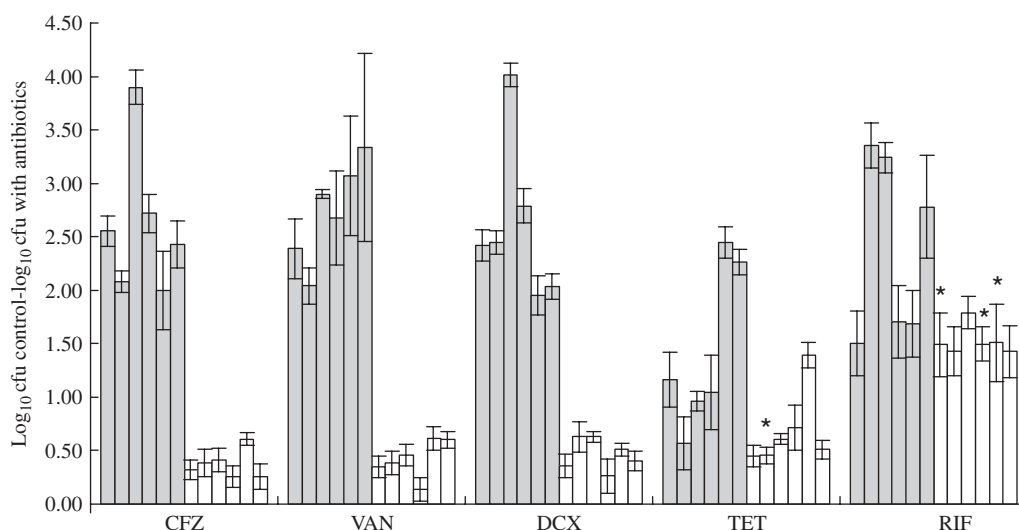
Figure 2. Mean fold reduction of cellular viability after 3 h of exposure to antibiotics. The y-axis indicates the difference in the \log_{10} cfu/mL between strains without antibiotic (controls) and strains treated with antibiotics (CFZ, cefazolin; VAN, vancomycin; DCX, dicloxacillin; TET, tetracycline; RIF, rifampicin), in planktonic cells (grey bars) and biofilm (white bars). Different bars represent different strains, from left to right: S. epidermidis 9142, IE186, M129, M187, S. haemolyticus IE246 and M176. *Indicates values that are not significantly different ( P > 0.05 , paired t -test).
